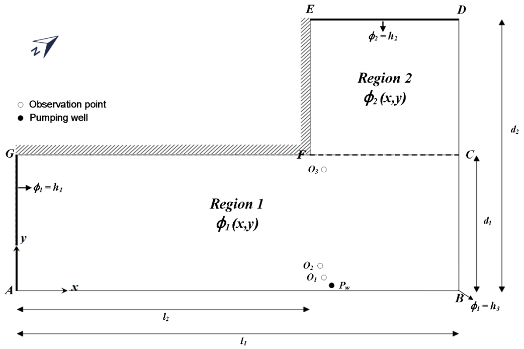
Figure 2: The L-Shaped fluvial aquifer with two sub-regions.
