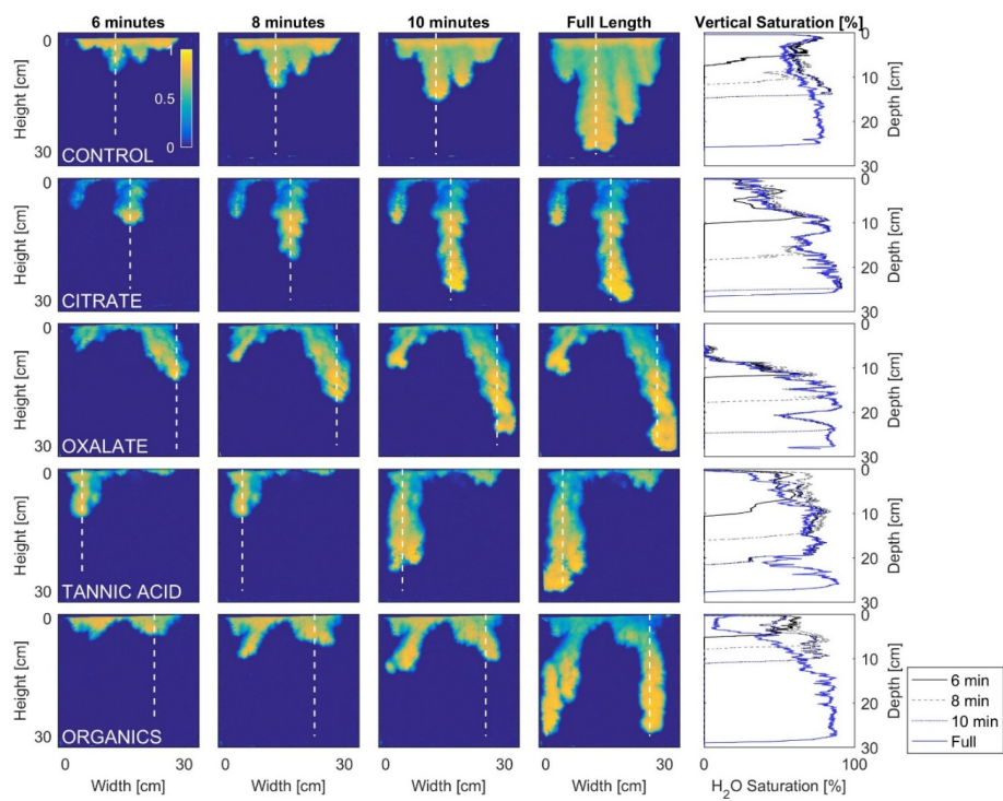
10 Figure 2A. Second tank experiment data set. Multigraph comparison of the dynamic vertical profiles of infiltration of water in U.S. Silica C778 ASTM graded sand for control (NaCl+HNS), and high concentrations of plant exudates (citrate and oxalate) and soil components (tannic acid and organics: Suwanee River Natural Organic Matter (SRNOM)). The images are of the main finger and the vertical water saturation profile analysis over time.
