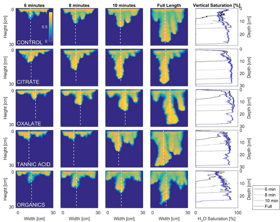
5 Figure 1A. Second tank experiment data set. Multigraph comparison of the dynamic vertical profiles of infiltration of water in U.S. Silica C778 ASTM graded sand for control (NaCl+HNS), and low concentrations of plant exudates (citrate and oxalate) and soil components (tannic acid and organics: Suwanee River Natural Organic Matter (SRNOM)). 10 The images are of the main finger and the vertical water saturation profile analysis over time.
