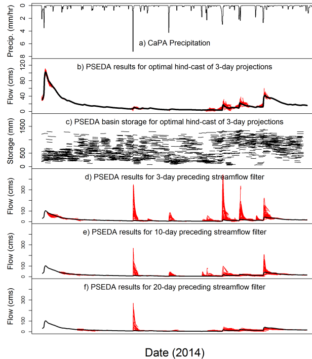
Figure 7. CaPA precipitation (a) for all simulations shown in this Figure. (b) Observed streamflow (black) and top 10 streamflow values (red) for the optimal hind-cast of 3-day projections. (c) Corresponding basin-wide storage values for the optimal hind-cast of 3-day projections. (d) Top 10 preceding streamflow filter projections for each of the 3-day filter periods. (e) Top 10 preceding streamflow filter projections for each of the 10-day filter periods. (f) Top 10 preceding streamflow filter projections for each of the 20-day filter periods. The black lines in (d), (e) and (f) show observed streamflow with different y-axis scaling than in (b).
