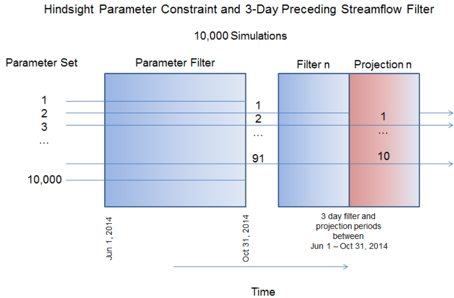
Figure 5. Schematic of the P-SEDA filter for the hindsight parameter constraint and preceding 3-day streamflow filter used in this study. 10,000 simulations are run continuously through the MESH model. The original 10,000 parameter sets are reduced to 91 parameter sets based on a hindsight analysis of parameters that are shown to be important during precipitation events between June 1 and October 31, 2014. These remaining 91 parameter sets are then selected for analysis in the preceding streamflow filter as if M = 91 in Algorithm 2.
