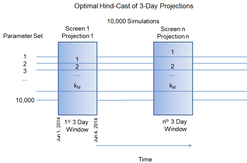
Figure 4. Schematic of P-SEDA P-SET for the optimal hindcast of 3-day projections used in this study. 10,000 simulations are run continuously through the MESH model, of which the screen chooses a number ( k_M ) for the hindcast analysis. The process is then repeated for subsequent screening periods.
