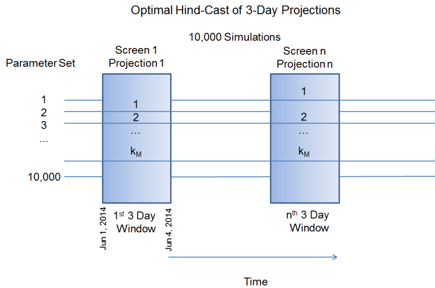
Figure 4. Schematic of the P-SEDA filter for the optimal hind-cast of 3-day projections used in this study. 10,000 simulations are run continuously through the MESH model, of which the filter screen chooses a number ( k_M ) for the hind-cast analysis. The process is then repeated for subsequent filter screening periods.
