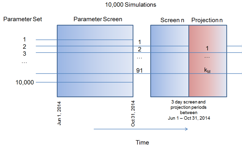
Figure 6. Schematic of the P-SEDA filter for the hindsight parameter constraint and preceding 3-day streamflow filter-screen used in this study. 10,000 simulations are run continuously through the MESH model. The original 10,000 parameter sets are reduced to 91 parameter sets based on a hindsight analysis of parameters that are shown to be important during precipitation events between June 1 and October 31, 2014. These remaining 91 parameter sets are then selected for analysis in the preceding streamflow filter-screen as if M = 91 in Algorithm 2.
