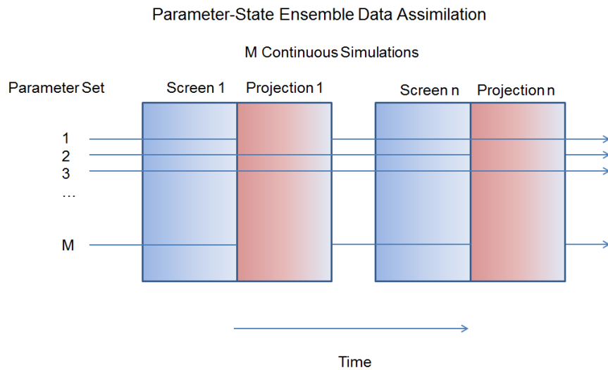
Figure 1. Schematic of the P-SEDA filter approach . M simulations are run continuously from a model, of which the filter screen chooses a number from which to analyze a projection. The process is then repeated for subsequent filter screening periods, noting that the M simulations run continuously through the previous projection periods even though they are not all selected for the previous projection period analysis.
