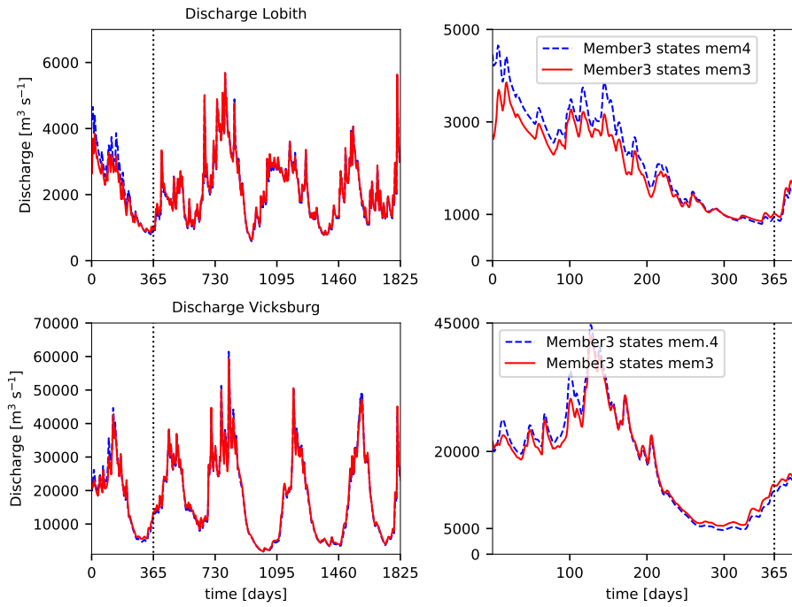
Fig. 1. Discharge at Lobith and Vicksburg from member3 of the EC-Earth T159 data initialized with spin-up states from member4 (blue) and member3 (red line). The right plots are a zoom in of the left figures.
