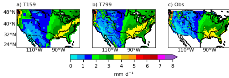
Fig. 3. 30-year average of daily precipitation sums (mm d-1) over the Mississippi basin for the low resolution EC-Earth simulations (T159), the high resolution EC-Earth simulations (T799) and the CPC dataset
