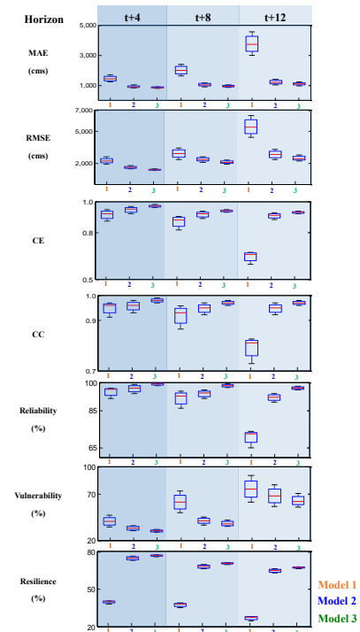
Figure 10 Sensitive analysis of the three models at horizon t+4, t+8 and t+12 in the testing period with cross-validation
