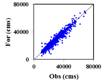
Figure 8 Scatter plots of the forecasted (For) and observed (Obs) values of reservoir inflow at horizons t+4, t+8 and t+12 in the testing period
