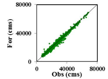
Figure 8 Scatter plots of the forecasted (For) and observed (Obs) values of reservoir inflow at horizons t+4, t+8 and t+12 in the testing period
