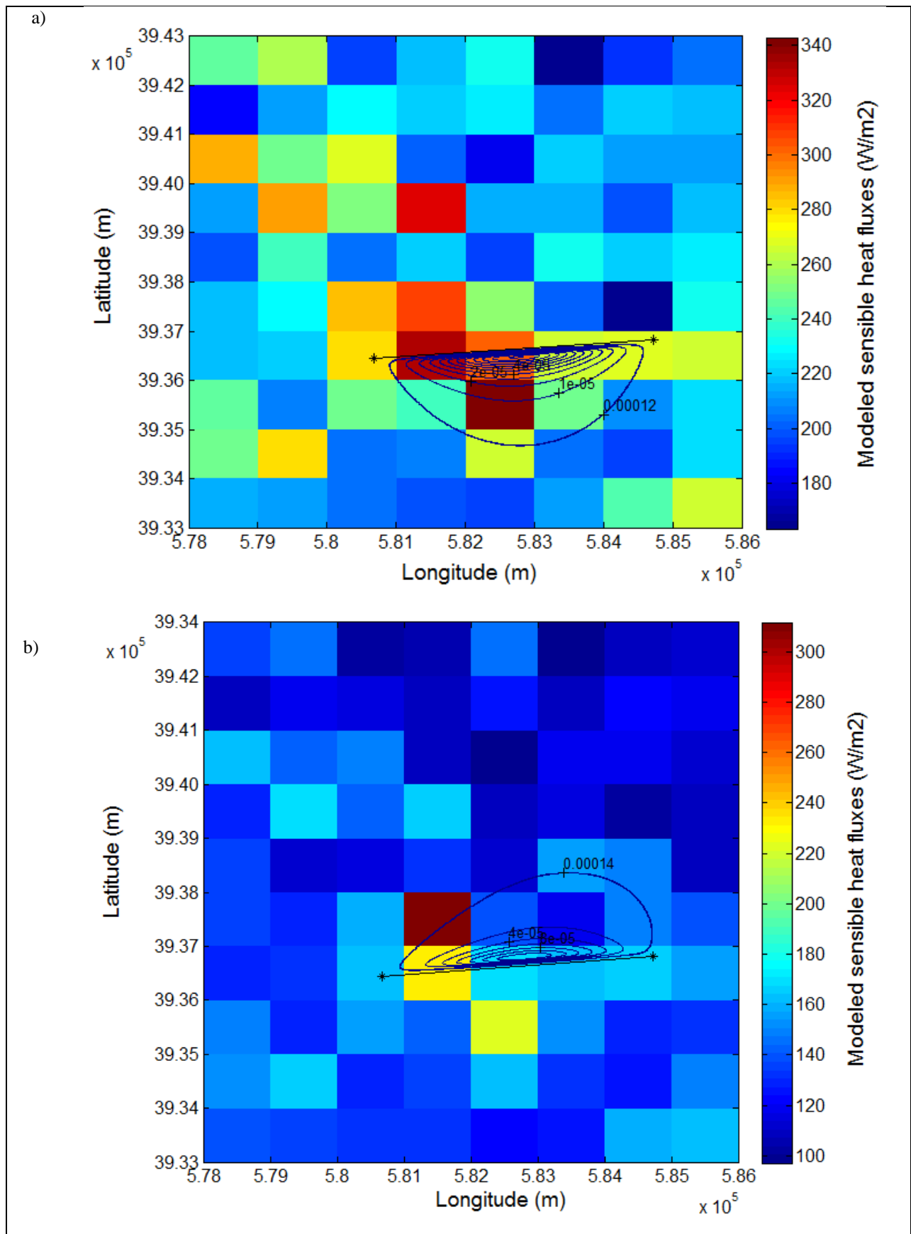
Figure 6: Model derived sensible heat fluxes and footprints for (a) DOY 2013-082 at Aqua time overpass and (b) DOY 2014-208 at Terra time overpass. The colored area shows the modeled flux and the contours shows the surface source area contributing to the scintillometer measurements.
