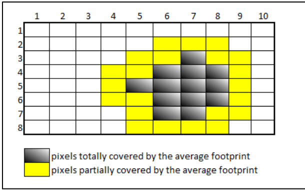
345 Figure 3 : MODIS pixels partially or totally covered by XLAS source area
