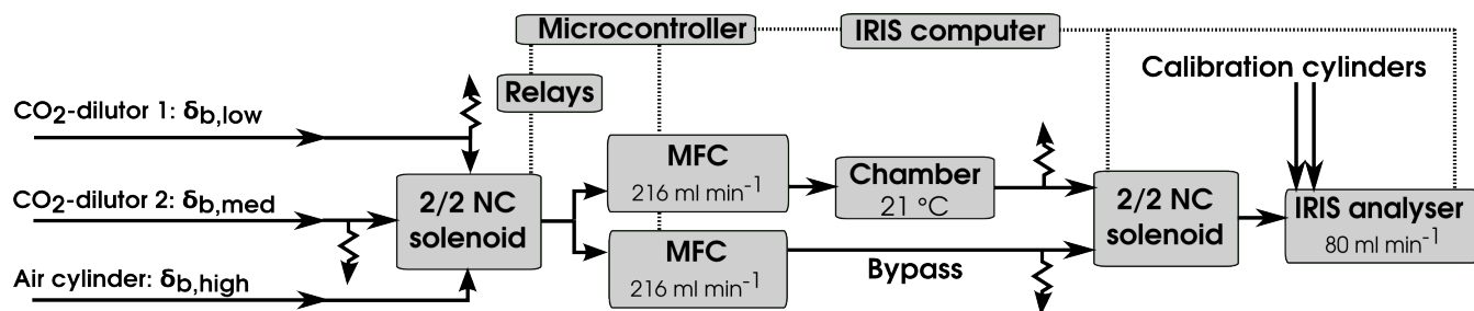
Figure 1: Schematic of the system used to make gas exchange measurements. Alternate measurements of the concentration and \delta^{18}\text{O} of \text{CO}_2 in chamber ( C_a , \delta_a ) and bypass lines ( C_b , \delta_b ) are made under three inlet conditions ( \delta_{b,low} , \delta_{b,med} , \delta_{b,high} ) that differ in terms of the \delta^{18}\text{O} of \text{CO}_2 .
