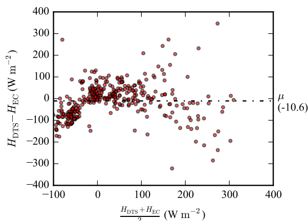
Figure 8. Tukey mean-difference plot comparing H_{EC} and H_{DTS} . With \mu = -10.6 \text{ W m}^{-2} , \text{RMSE} = 82 \text{ W m}^{-2} . (15 minute averages). Data from 10, 12-14, 19-22, and 28-30 August 2016.
