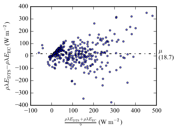
Figure 7. Tukey mean-difference plot comparing \rho\lambda E_{EC} and \rho\lambda E_{DTS} . With \mu = 18.7 \text{ W m}^{-2} , \text{RMSE} = 90 \text{ W m}^{-2} . (15 minute averages). Data from 10, 12-14, 19-22, and 28-30 August 2016.
