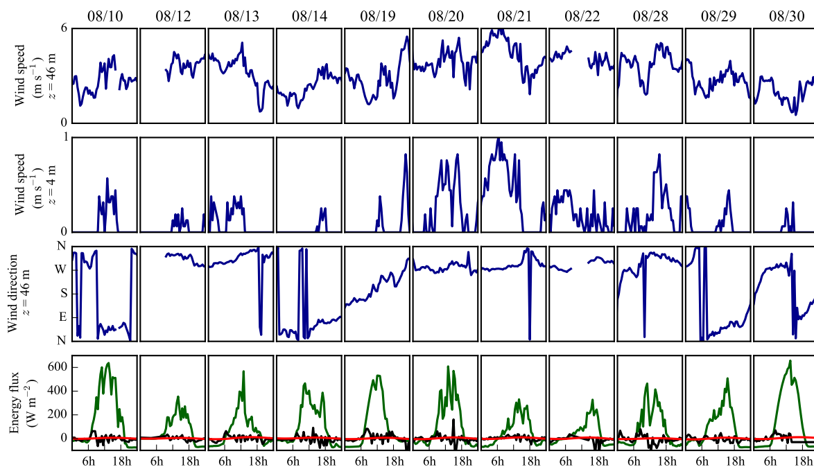
Figure 3. Meteorological conditions during the days that both DTS and eddy covariance data was available. From top to bottom: wind speed at the top of the tower, wind speed at the bottom of the tower, wind direction at the top of the tower, and the measured energy fluxes (green: net radiation, red: soil heat flux, black: energy storage change \frac{dQ}{dt} ).
