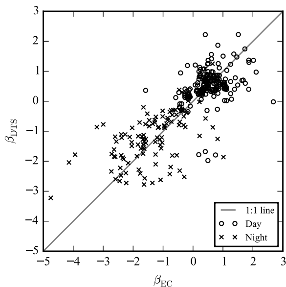
Figure 5. Correlation between the DTS measured ( \beta_{DTS} ) and eddy covariance measured ( \beta_{EC} ) Bowen ratios. Daytime data is between 7:00 and 18:00. Data from 10, 12-14, 19-22, and 28-30 August. R^2=0.59 . RMSE=0.81 . n = 319 data points.
