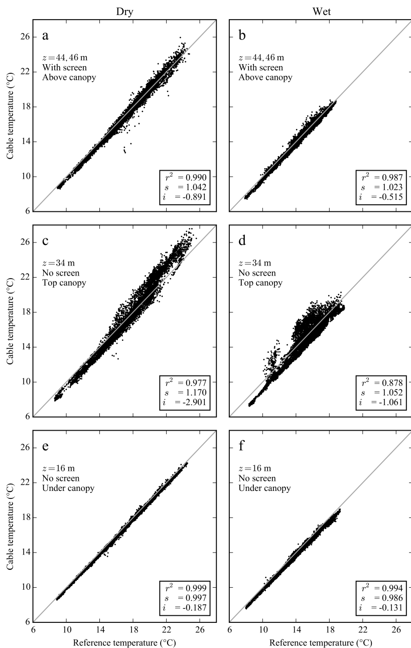
Figure 4. Comparison between the 6 mm DTS cable and reference temperatures. Grey line shows 1:1 correlation. Data from 10-23 August 2016. a: Dry cable at 44 m and reference air temperature at 46 m, the cable is shielded by the screen. b: Wet cable at 44 m and reference wet-bulb temperature at 46 m, the cable is shielded by the screen. c: Dry cable and reference air temperature at 34 m, the cable is exposed to direct sunlight. d: Wet cable and reference wet-bulb temperature at 34 m, the fibre optic cable is exposed to direct sunlight. e: Dry cable and reference air temperature at 16 m, under the canopy so less direct sunlight hits the fibre optic cable. f: Wet cable and reference wet-bulb temperature at 16 m, under the canopy so less direct sunlight hits the fibre optic cable. Shown are the linear correlation coefficients; the coefficient of determination ( r^2 ), the slope ( s ), and the intercept ( i ).
