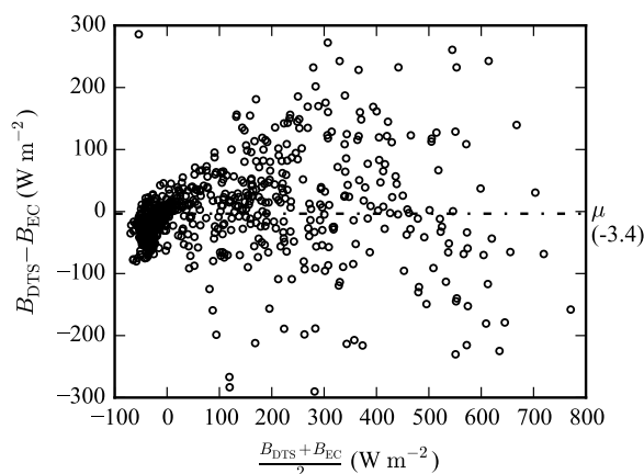
Figure 6. Tukey mean-difference plot comparing B_{DTS} and B_{EC} . With \mu = -3.4 \text{ W m}^{-2} , \text{RMSE} = 76 \text{ W m}^{-2} , n = 741 data points. (15 minute averages). Data from 10, 12-14, 19-22, and 28-30 August 2016.
