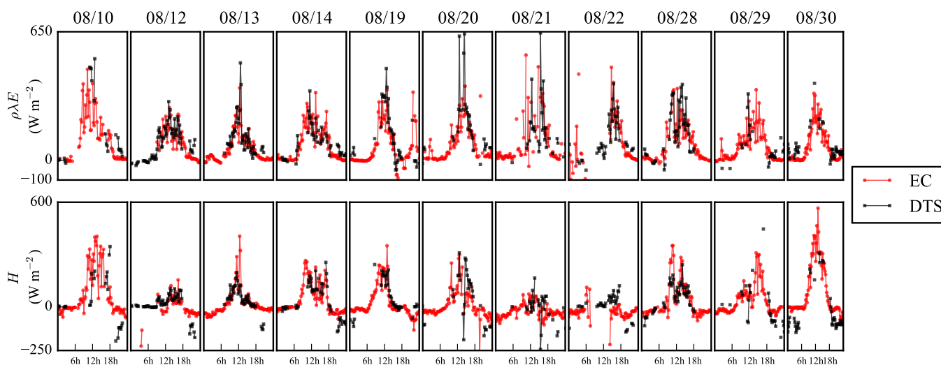
Figure 9. Plot comparing the BR-DTS and EC measured sensible ( H ) and latent ( \rho\lambda E ) heat fluxes over time. (15 minute averages). Data from 10, 12-14, 19-22, and 28-30 August 2016.
