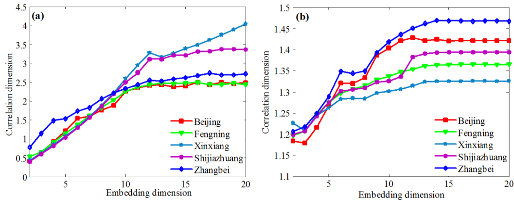
Figure 7: Variation of correlation dimension versus embedding dimension of climate variables: (a) precipitation and (b) air temperature.
