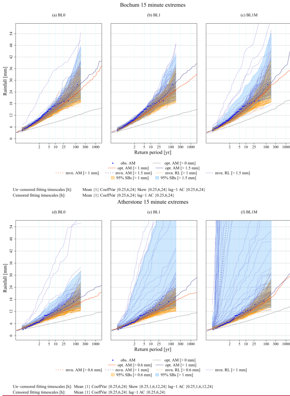
Figure 10 , Change in 95% simulation bands (SBs) and mean of the MVN realisations (mvn. AM) for Bochum and Atherstone 15 minute data with well identified ( > 1.0 mm and > 0.6 mm) and poorly identified ( > 1.5 mm and > 1.0 mm) censored model parameters. The spread of the individual realisations is also shown with solid lines (mvn. RL).
