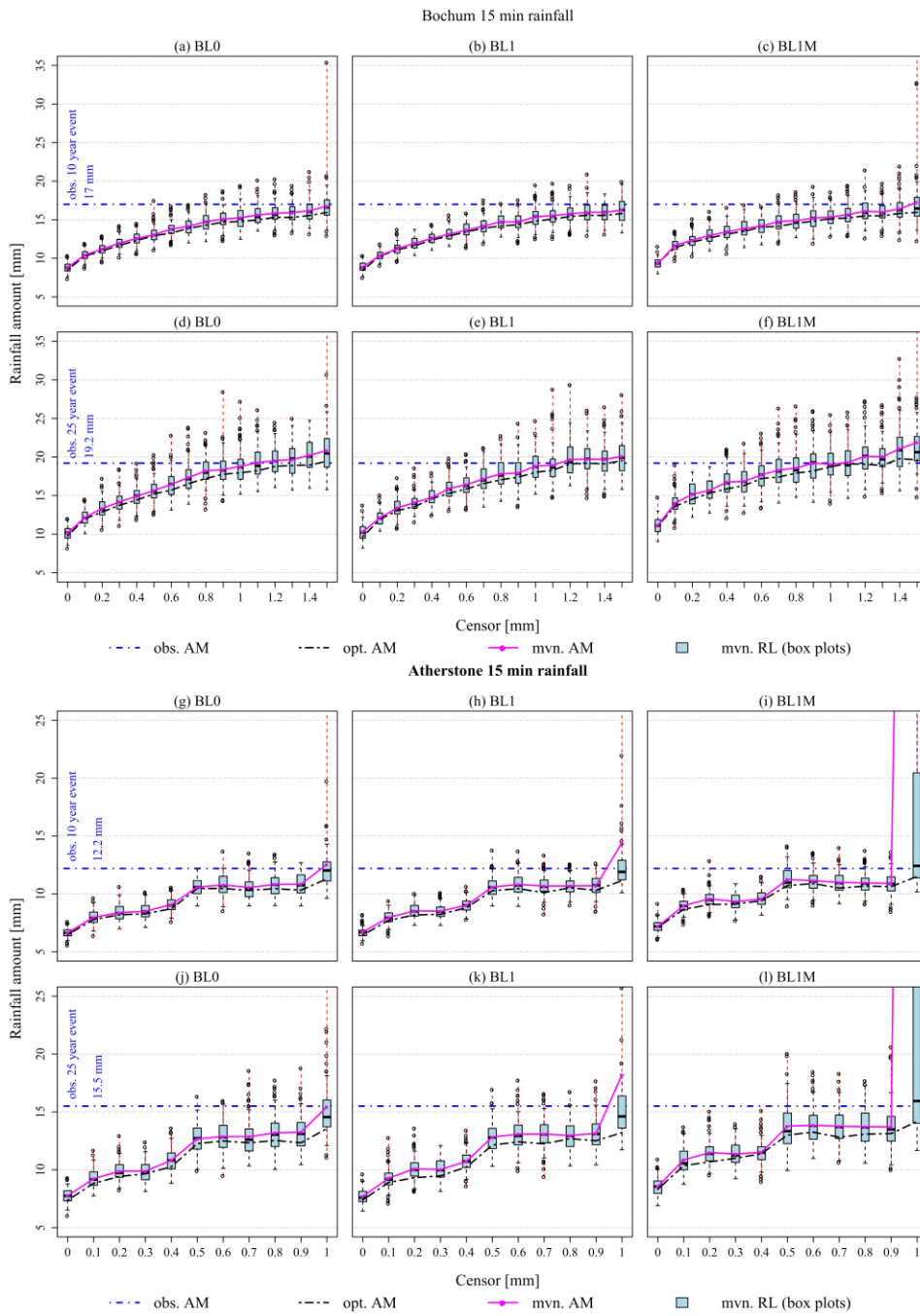
Figure 12. Variation in extreme value estimation with censor for 15 minute data at Bochum and Atherstone for two annual return periods: 10 and 25 years. Plots show the optimal realisations (opt. AM), the mean of the MVN realisation (mvn. AM) and the spread of the individual realisations (mvn. RL) with box plots.
