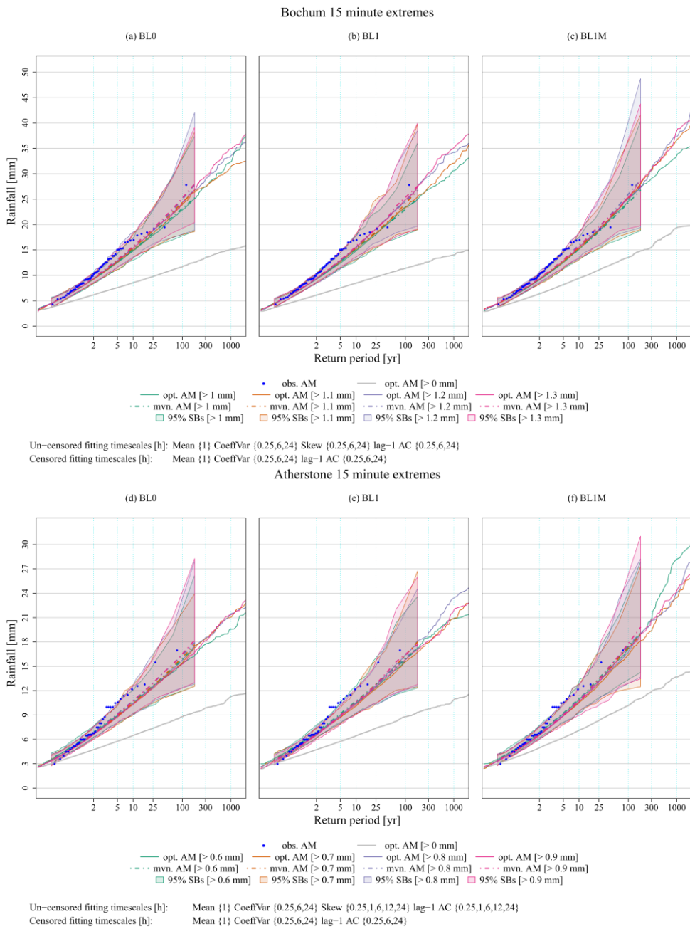
Figure 5. Extreme value estimation at 15 minute resolution. Optimal realisations (opt. AM) are shown with solid lines and the mean of the MVN realisation (mvn. AM) are shown with dashed lines. Simulation bands (SBs) are shown with filled polygons.
