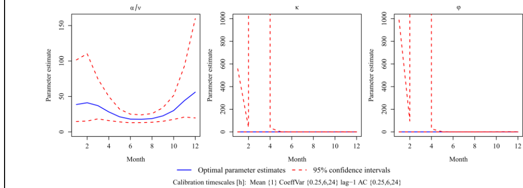
Figure 11. Fitted model parameters for the BLIM model with 1.5 mm censor applied to Bochum 15 minute data.
