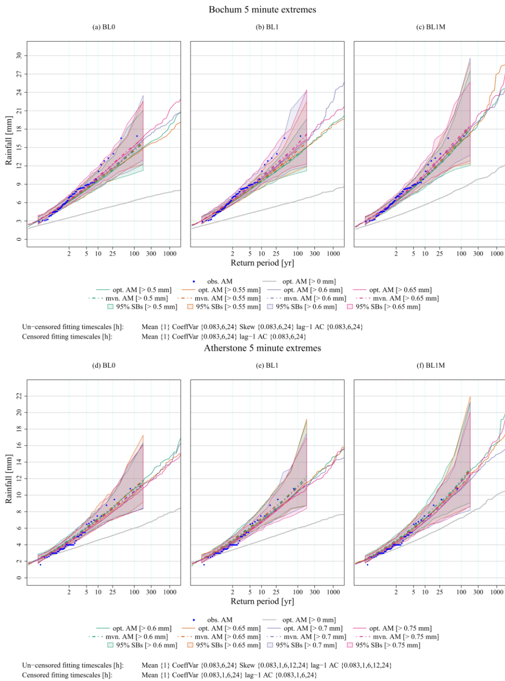
Figure 4. Extreme value estimation at 5 minute resolution. Optimal realisations (opt. AM) are shown with solid lines and the mean of the MVN realisation (mvn. AM) are shown with dashed lines. Simulation bands (SBs) are shown with filled polygons.
