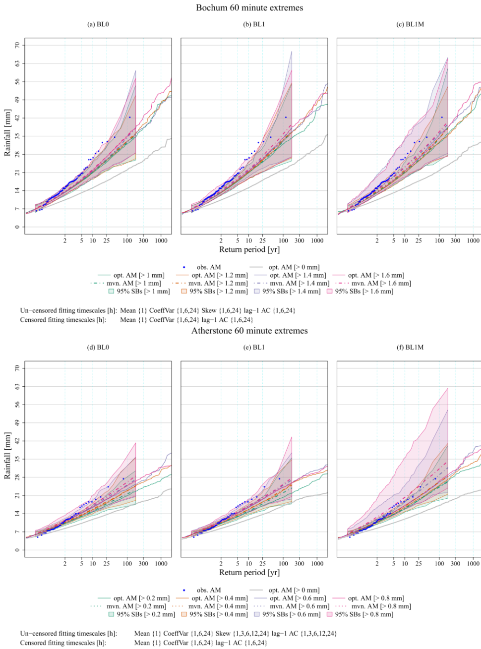
Figure 6 Extreme value estimation at 60 minute resolution. Optimal realisations (opt. AM) are shown with solid lines and the mean of the MVN realisation (mvn. AM) are shown with dashed lines. Simulation bands (SBs) are shown with filled polygons.
