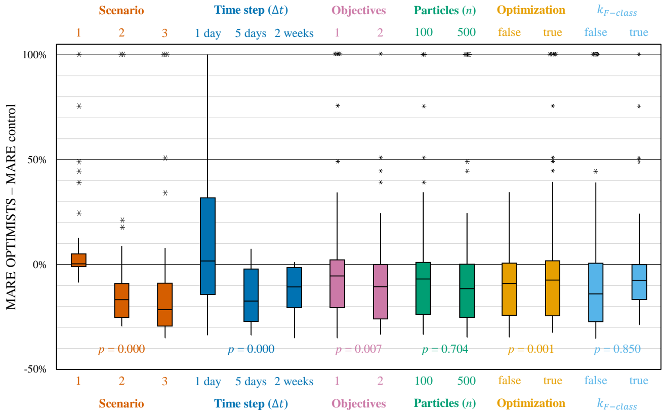
5 Figure 3. Boxplots of the changes in forecasting error (MARE) achieved while using OPTIMISTS on Experiment 1 (Blue River). Changes are relative to an open-loop control run where no assimilation was performed. Each column corresponds to the distribution of the error changes on the specified scenario or assignment to the indicated parameter. Positive values indicate that OPTIMISTS increased the error, while negative values indicate it decreased the error. Outliers are noted as asterisks and values were limited to 100%. For the one-objective case the particles' MAE was to be minimized; for the two-objective case, the likelihood given the background was to be maximized in addition. No optimization ("false") corresponds to p_{\text{samp}} = 1.0 (i.e., all samples are obtained from the prior distribution); "true" corresponds to p_{\text{samp}} = 0.25 . The p -values were determined using ANOVA (Montgomery, 2012), and indicate the probability that the differences in means corresponding to boxes of the same colour are produced by chance (e.g., values close to zero indicate certainty that the parameter effectively affects the forecast error). 10
