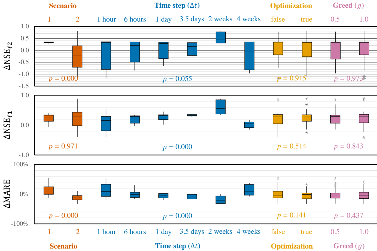
5 Figure 6. Boxplots of the changes in forecasting performance ( NSE_{\ell_2} , NSE_{\ell_1} , and MARE) achieved while using OPTIMISTS on Experiment 3 (Indiantown Run). Changes are relative to an open-loop control run where no assimilation was performed. Each column corresponds to the distribution of the error metric changes on the specified scenario or assignment to the indicated parameter. Positive values indicate improvements for the NSE_{\ell_2} and the NSE_{\ell_1} . See the caption of Fig. 3 for more information.
