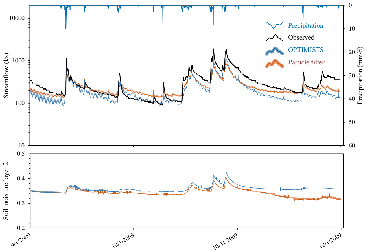
5 Figure 7. Comparison of four-day lead time probabilistic streamflow (top) and area-averaged soil moisture (bottom) forecasts between OPTIMISTS ( \Delta t = 7 days, 2 objectives, n = 50 , no optimization, and D-class kernels) and a traditional PF ( n = 50 ) for the Indiantown Run. The dark blue and orange lines indicate the mean of OPTIMISTS' and the PF's ensembles respectively, while the light blue and light orange bands illustrate the spread of the forecast by highlighting the areas where the probability density of the estimate is at least 50% of the density at the mode (the maximum) at that time step. The green bands indicate areas where the light blue and light orange bands intersect. Layer 2 of the soil corresponds to 100 to 250 mm depths.
