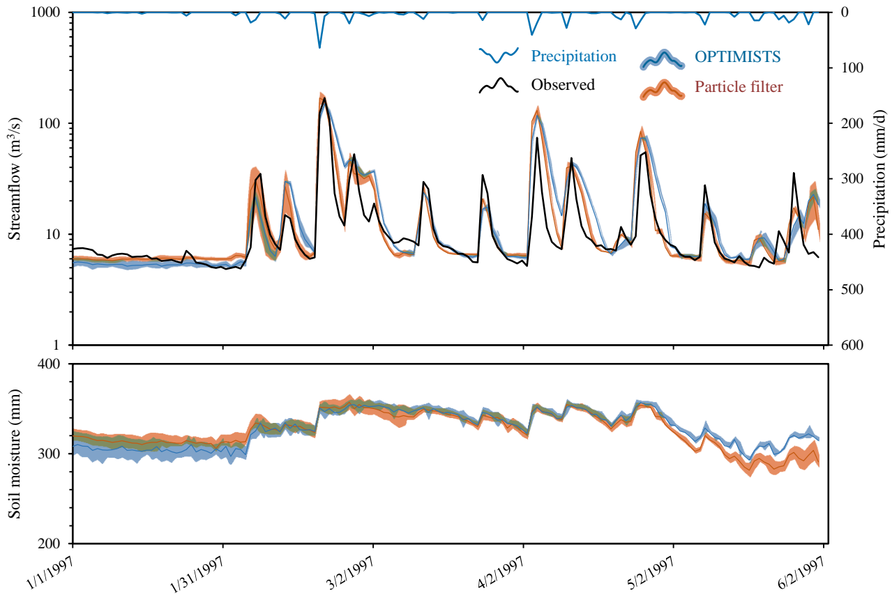
5 Figure 4. Comparison of six-day lead time probabilistic streamflow (top) and area-averaged soil moisture (bottom) forecasts between OPTIMISTS ( \Delta t = 7 days; 3 objectives: NSE_{\ell_2} , MARE, and likelihood; n = 30 ; no optimization, and D-class kernels) and a traditional PF ( n = 30 ) for the Blue River. The dark blue and orange lines indicate the mean of OPTIMISTS' and the PF's ensembles respectively, while the light blue and light orange bands illustrate the spread of the forecast by highlighting the areas where the probability density of the estimate is at least 50% of the density at the mode (the maximum) at that time step. The green bands indicate areas where the light blue and light orange bands intersect.
