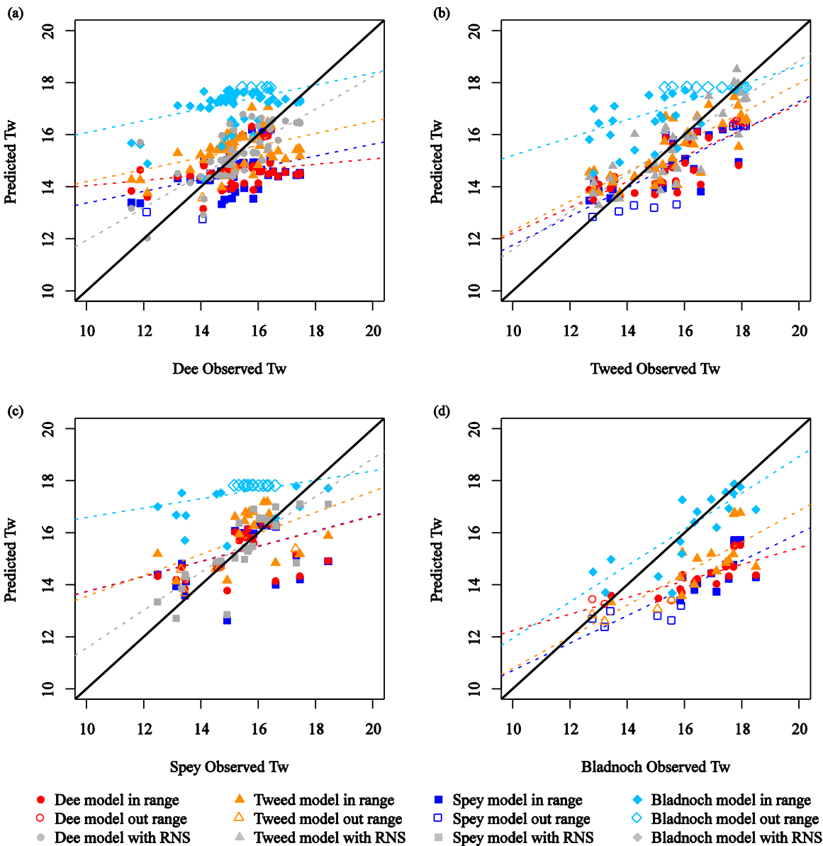
Figure 5. LS model transferability. Panels a, b, c, d show predicted Tw_{max} when the target catchment is the Dee, Tweed, Spey and Bladnoch respectively. The colours and symbols indicate the donor catchment: Dee (red circles), Tweed (orange triangles), Spey (dark blue squares) and Bladnoch (light blue diamonds). Filled (open) symbols indicate sites in (out) of the environmental range of the donor catchment. When the target and donor catchments are the same, the coloured points are based on predictions using only covariates; the grey symbols show the corresponding predictions based on the covariates and the RNS. The dashed lines are robust regression lines of observed against predicted values. Models which transfer well have points falling close to the 1:1 line.
