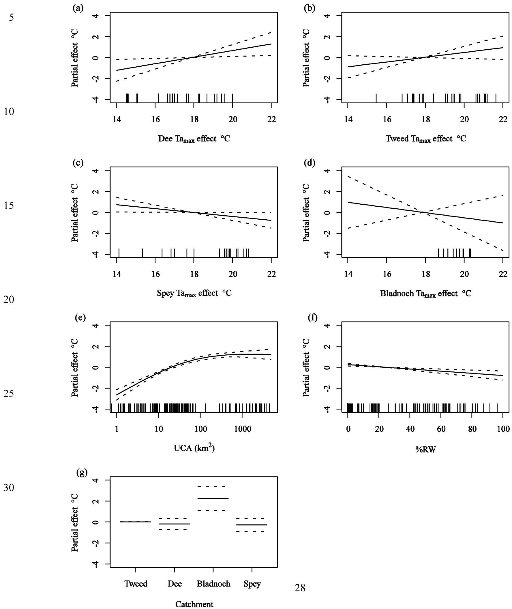
Figure 8. Multi-catchment LS_Ta model effects with pointwise 95% confidence bands: a) Dee Ta max , b) Tweed Ta max , c) Spey Ta max , d) Bladnoch Ta max , e) UCA, f) %RW, g) Catchment.
