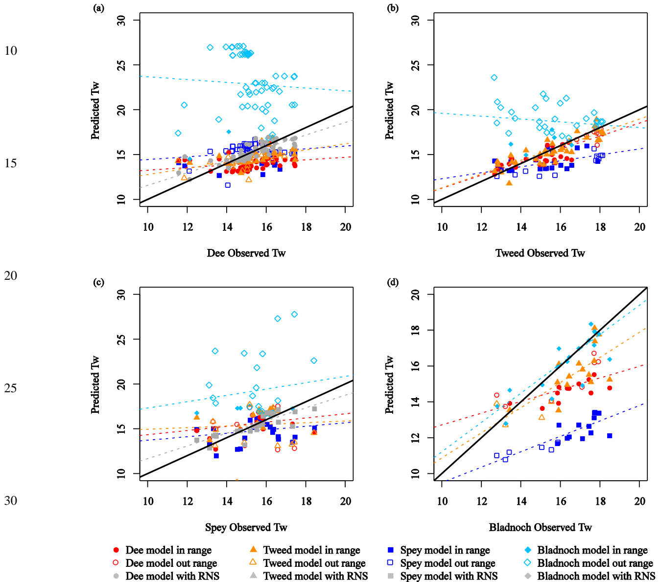
Figure 6. LS-Ta model transferability. Panels a, b, c, d show predicted Tw_{max} when the target catchment is the Dee, Tweed, Spey and Bladnoch respectively. The colours and symbols indicate the donor catchment: Dee (red circles), Tweed (orange triangles), Spey (dark blue squares) and Bladnoch (light blue diamonds). Filled (open) symbols indicate sites in (out) of the environmental range of the donor catchment. When the target and donor catchments are the same, the coloured points are based on predictions using only covariates; the grey symbols show the corresponding predictions based on the covariates and the RNS. The dashed lines are robust regression lines of observed against predicted values. Models which transfer well have points falling close to the 1:1 line.
