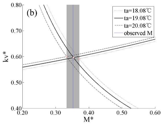
Figure 6: M^* changes with precipitation ( P_\tau ) and air temperature ( t_a ) ((a) ~ (b) grassland; (c) ~ (d) forest). The shaded areas mean the range of M^* with the change of vegetation properties.
