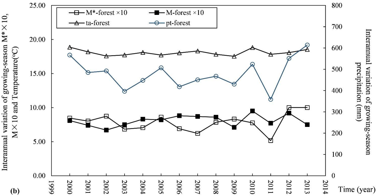
Figure 4: Variation of M^* , M during precipitation ( P_t ) and air temperature ( t_a ) during 2000-2013 ((a) grassland; (b) forest).
