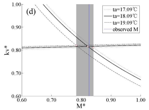
Figure 6: M^* changes with precipitation ( P_\tau ) and air temperature ( t_a ) ((a) ~ (b) grassland; (c) ~ (d) forest). The shaded areas mean the range of M^* with the change of vegetation properties.
