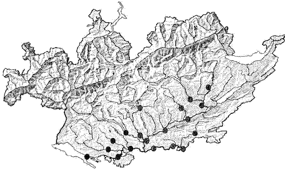
Figure 21: Contribution (green dots) and non-contribution (red dots) of rivers to particular pre-instrumental minor flood events.
