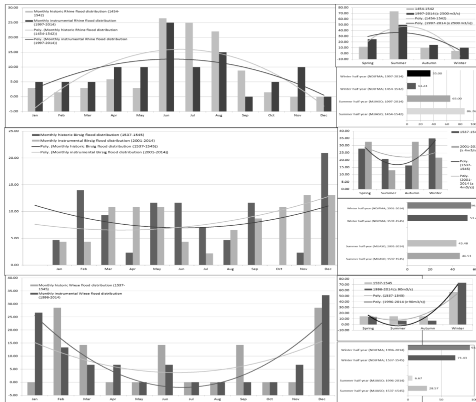
Figure 17: Distribution of historical and instrumental Rhine, Birsig and Wiese flood events in comparison
