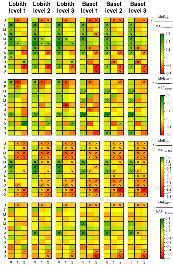
Figure 3. MAE skill score of the S4PT model with respect to the climatology, the preMet and subMet models, and bias corrected H-TESEL runoff. The ordinate depicts the calendar month and the abscissa the monthly lead time. Crosses indicate p-values smaller than 0.05 for the null hypothesis ‘the reference model in the denominator and the S4PT model score an equal mean absolute error’; n = 30 .
