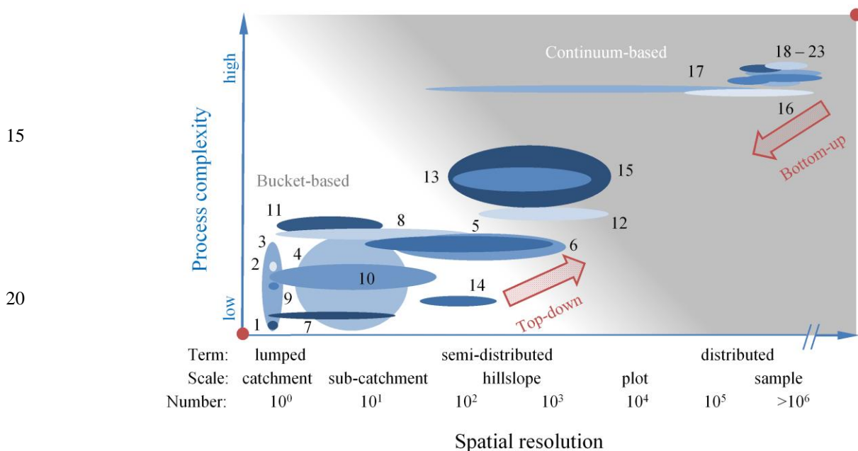
Figure 1: Conceptual sketch of approximate positions of a selection of typical applications of frequently used catchment-scale models on the spatial resolution – process complexity continuum, compared to a selection of observation variables and their availability to force and constrain models. The Spatial resolution axis shows approximate ranges of numbers and associated scales of individual spatial units (e.g. grid cells) within the model domain (e.g. catchment) for typical applications of the individual models. The Process complexity axis indicates the number of individual processes/processes within one spatial unit. The increasingly grey shaded area indicates the transition from bucket-based (white) to continuum-based models. The red dots indicate the two endpoints along the resolution-complexity continuum. Models: 1 – Unit hydrograph (Sherman, 1932), 2 – HBV (Bergström, 1992), 3 – SUPERFLEX (Fenicia et al., 2011), 4 – FLEX-Topo (Gharari et al., 2014a), 5 – mhM (Samaniego et al., 2010), 6 – mhM-topo (Nijzink et al., 2016a), 7 – SWAT (Arnold et al., 1998), 8 –
