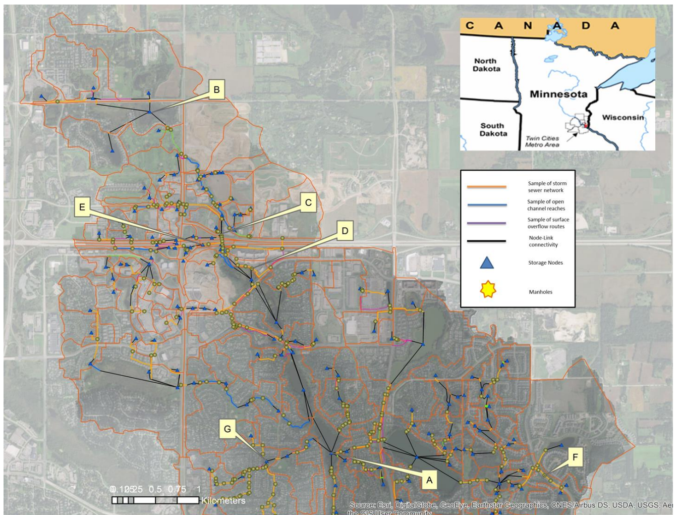
Figure 1 Location of the model and the sub-watersheds along with the reference points used in the discussion below. The details of the reference points and further explanation are presented in Table 1. The Orange links are example of the sewer network geometry in the model. The blue links represent
