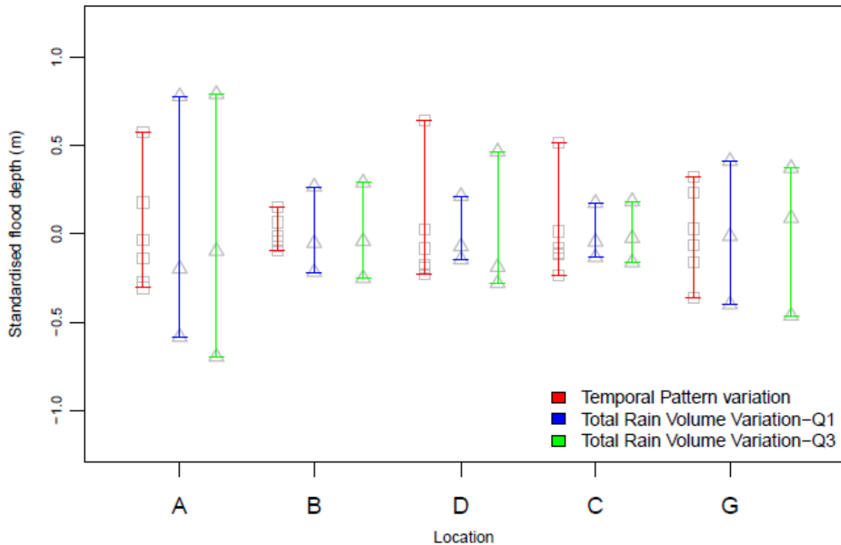
Figure 7 Comparison of total volume of rainfall and temporal patterns variability impact on peak flood depth. Flood depth variation due to the 6 different temporal patterns with 160 mm of rain compared to 110, 160 and 210 mm of total rainfall over 24 hours distributed over Q1-50 and Q3-50 temporal patterns. Flood depths were standardised by subtracting the mean at each location for ease of comparison.
