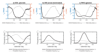
Figure 4. Examples of the annual variation of the model parameters. The parameters are calculated for 90 days intervals beginning at the calendar day for which the value is plotted. Top row: residence time \tau_r and mean daily precipitation depth \alpha ; bottom row: precipitation frequency \lambda_p and discharge-producing frequency \lambda . The plots have different y-axis scales.
