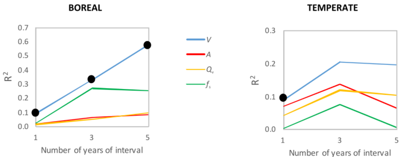
5 Figure 8: Performance of forest attributes as predictors of the residual of the evaporative ratio. Coefficients of determination ( R^2 ) of the linear regressions between the residual of the evaporative ratio, (E/P)_r , and the forest attributes of forest biomass ( V ), forest cover ( A ), forest composition ( Q_v ) and fraction of precipitation falling as snow ( f_s ), in the boreal and temperate basin groups. The Pearson coefficient of determination ( R^2 ) is shown for the regressions using annual ( N=52 ), three-year ( N=17 ) and five-year means ( N=10 ) during the period 1961-2012, with N being the number of values available for each regression with each interval selection. The significance ( p<0.05 ) of the R^2 of each linear regression is shown with a black dot. See Table S1 in Supplementary materials for values.
