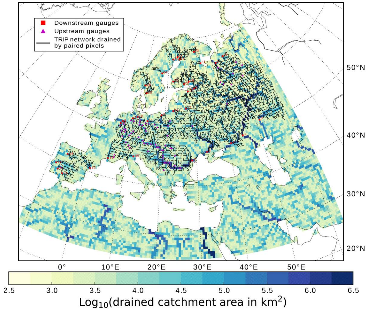
5 Figure 1: Selected GRDC discharge gauges and corresponding drained CTRIP river network. The colour map categorises reflect the logarithm of the upstream catchment area of each pixel. The numbers associated to downstream gauges are sorted by descending upstream area and refer to the index N in Fig. 2. For readability, gauges are mapped on the paired pixel.
