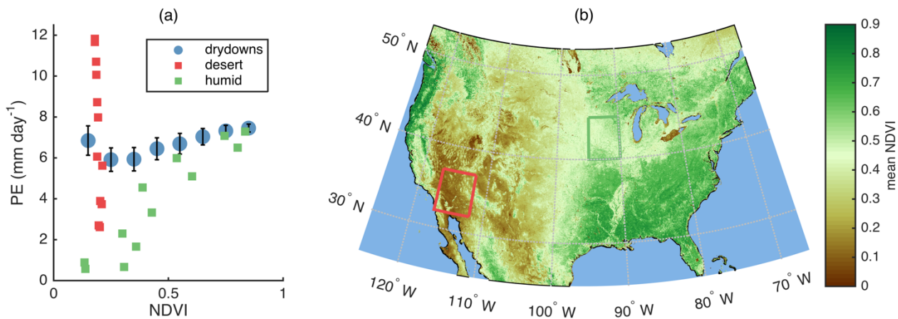
20 Figure 8: (a) Circles show median PE as a function of 8 equal-width bins of increasing NDVI for all drydowns used in this study. Squares show average monthly relationships between PE and NDVI in two regions. (b) Extent indicators show locations of two regions.
