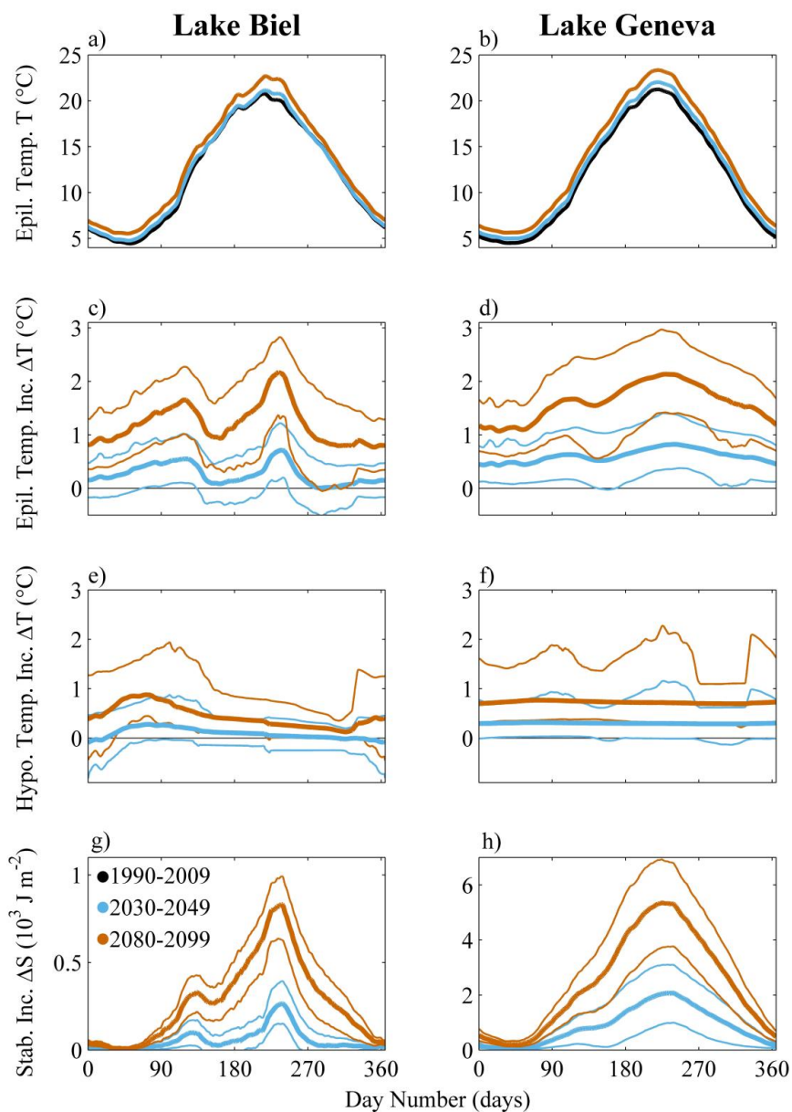
794 Figure 7. Modeled climate impact from scenarios LB3 (LB, left column) and LG3 (LG, right column) displayed 795 as daily mean (thick lines) and maximum/minimum model values (thin lines) for near-future (blue, 2030-2049) 796 and far-future (orange, 2080-2099) time periods relative to the reference period (black, 1990-2009). 797 Anthropogenic MNPP heat input entering LB has been excluded from near-future and far-future time periods but
