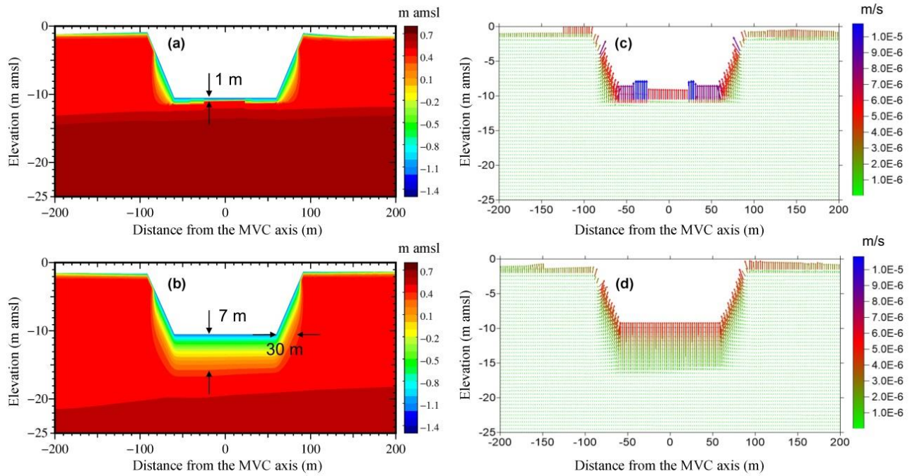
Figure 11: Computed (a,b) pressure distribution and (c,d) velocity field at the maximum wake induced by the Cargo-Hazard A ship transit in (a,c) Section-1 and (b,d) Section-2. The dimensions of the subsurface portion feeling the ship transit are highlighted in (a,b). Vertical exaggeration is 8.
