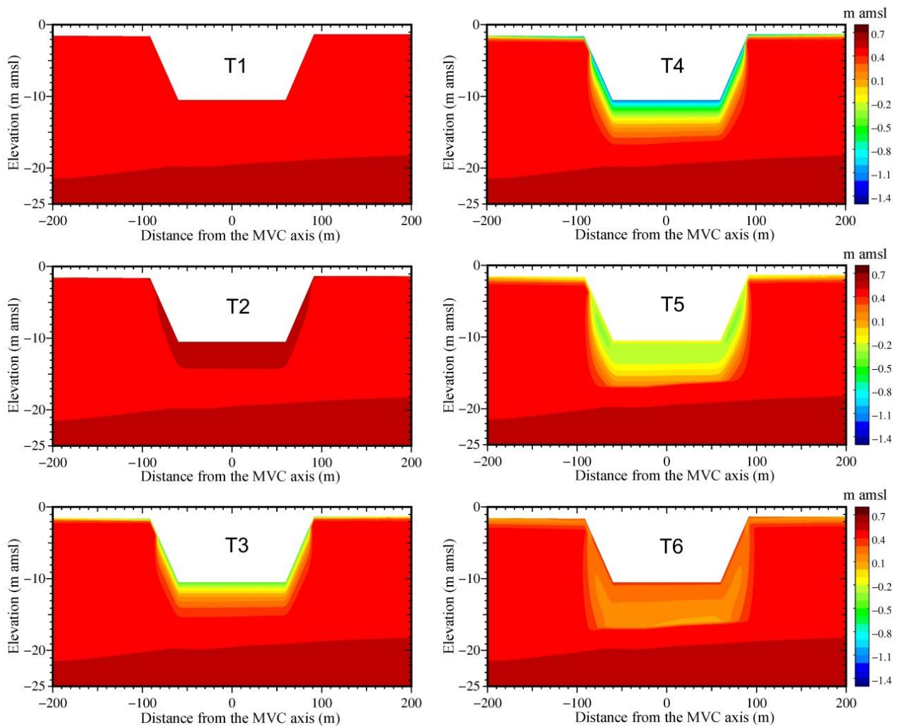
Figure 10: Section-2: computed pressure distribution at the times T1-T6 highlighted in Fig. 4a during the transit of the Cargo-Hazard A cargo liner of Fig. 4b. The vertical exaggeration is 8.
