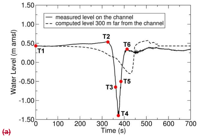
Figure 4: (a) Water level (m above msl) recorded on the bottom of the MMIC and computed by SHYFEM on the tidal flat 300 m far from the channel caused by the transit on April 6, 2016, of the Cargo-Hazard A. A photo of the vessel is shown in (b). The commercial vessel, which was used as reference, is 280 m long, 40 m wide, and characterized by a gross tonnage of 66433 t. The ship speed s was equal to 8.1 knots (4.2 m/s). The time steps T1-T6 highlighted by red dots in (a) refer to the model outcome shown in Fig. 10.
