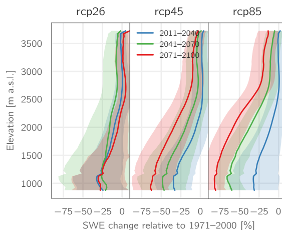
Figure 9. Elevation-dependent projected change in SWE (multi-model means, shadings indicate \pm one standard deviation) relative to the period 1971–2000 for the RCPs 2.6, 4.5, and 8.5.
