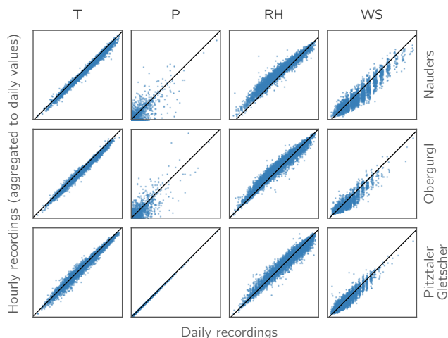
Figure 18. Scatter plots of daily vs. aggregated hourly recordings of air temperature (T), precipitation (P), relative humidity (RH), and wind speed (WS) for three stations in the study area.
