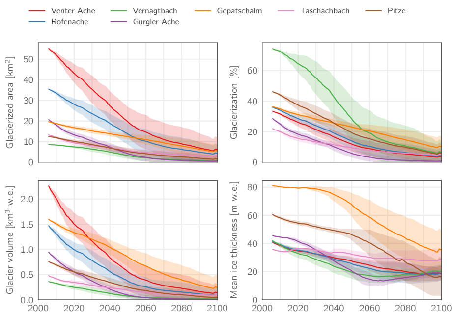
Figure 13. Evolution of the absolute (top left) and relative (top right) glacierized area for each catchment in the RCP4.5 scenario, as well as the absolute glacier volume (bottom left) and the mean ice thickness (bottom right). Note that the latter is calculated only over the glacierized fraction of the catchment and not the entire catchment area (i. e., it is the result of dividing the bottom left plot by the top left plot). Lines and shadings represent multi-model means \pm one standard deviation.
