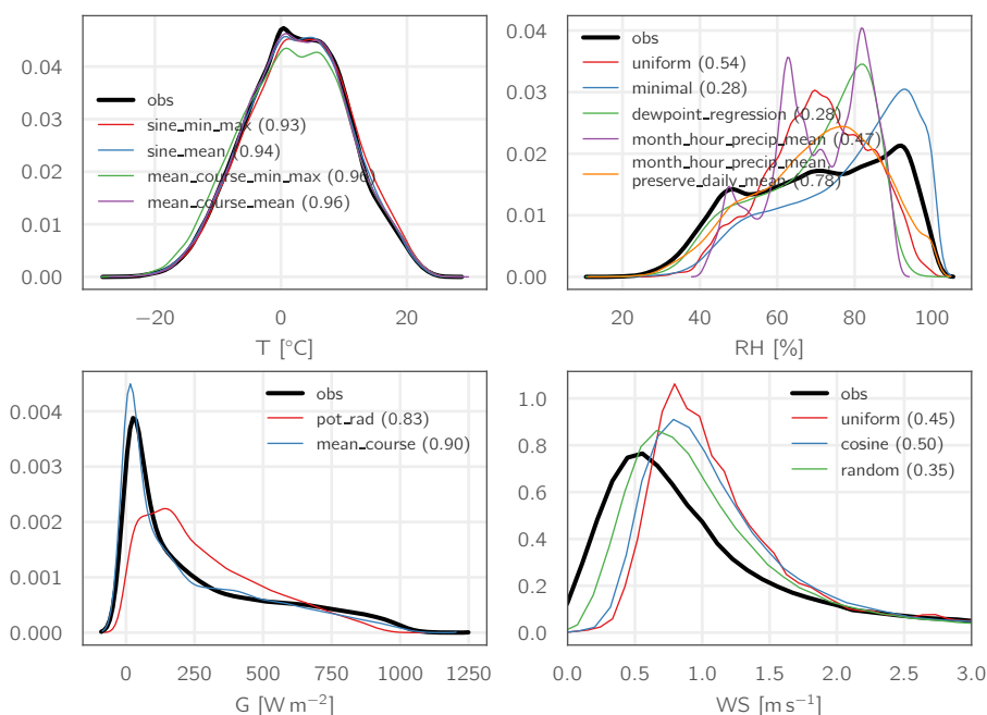
Figure 6. Density functions of the observed hourly values (black lines) for station Obergurgl (period 1999–2013) and the respective aggregated-and-disaggregated values using different disaggregation methods for the variables temperature, relative humidity, global radiation, and wind speed. Numbers in parentheses indicate the R^2 of the regression against the observations.
