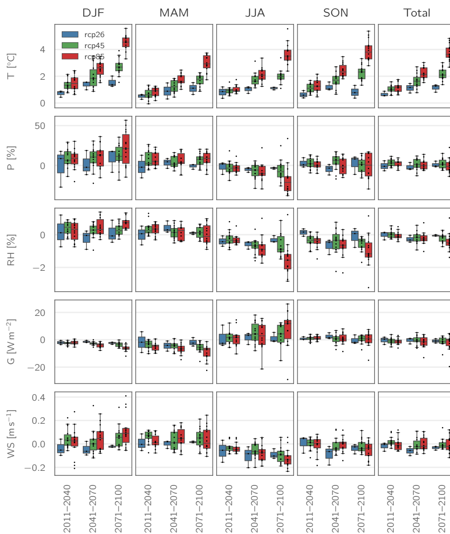
Figure 7. Projected seasonal changes for temperature (T), precipitation (P), relative humidity (RH), global radiation (G), and wind speed (WS) according to the selected EURO-CORDEX scenario simulations (spatial averages over the study area; changes calculated relative to 1971–2000). Small dots represent the individual GCM-RCM realizations.
