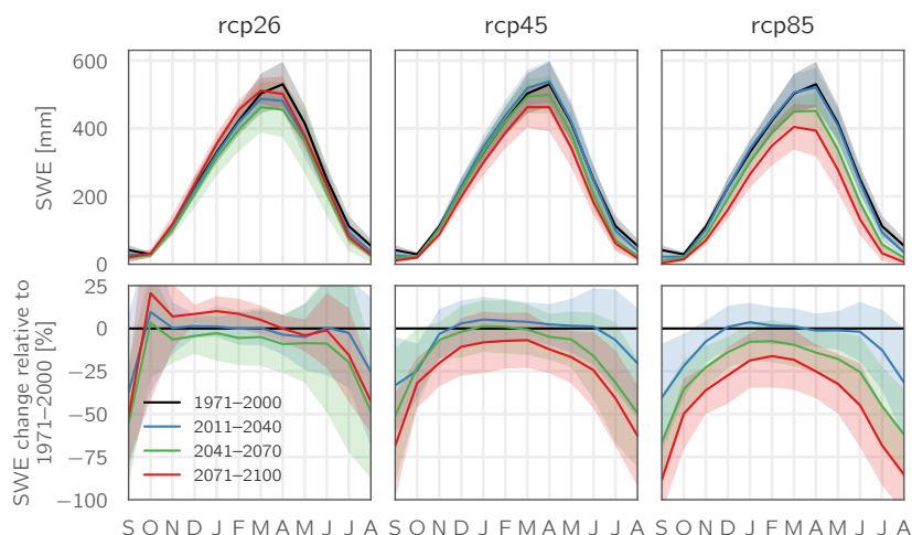
Figure 10. Mean monthly SWE (multi-model means, shadings indicate \pm one standard deviation) over the entire study area (Fig. 1) for the three RCPs (top) and relative changes compared to 1971–2000 (bottom).
