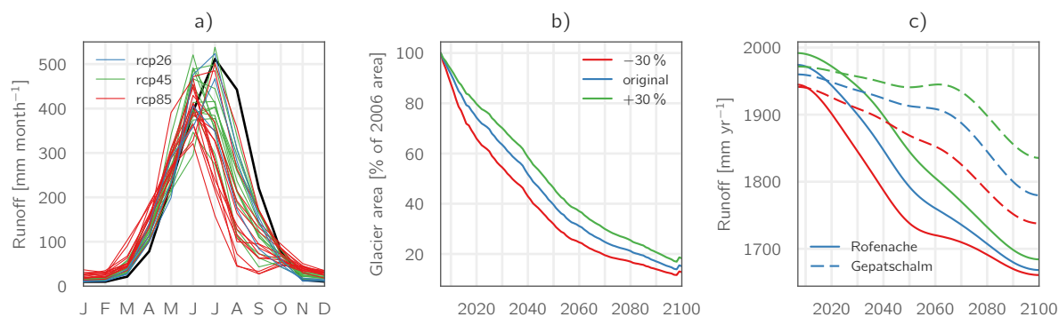
Figure 21. a) Average monthly runoff (period 2071–2100) for the Pitze catchment as simulated for all 31 individual GCM-RCM realizations, b) evolution of the total glacierized area for the entire Ötztal Alps study site as simulated by altering the initial ice thickness distribution by \pm 30\% (multi-model mean values for the RCP4.5 scenario), and c) corresponding runoff evolution (10-year Gaussian low-pass filtered) for the Rofenache and Gepatschalm catchments.
