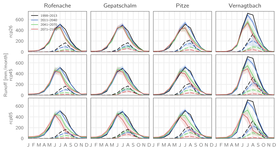
Figure 15. Average monthly runoff (multi-model mean \pm one standard deviation indicated as shaded bands) as simulated for the early, middle, and late 21st century for four catchments and the three emission scenarios. Dashed lines indicate bare ice melt runoff.
