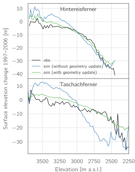
Figure 3. Observed and simulated glacier surface elevation change during the period 1997–2006 as a function of elevation for the glaciers Hintereisferner and Taschachferner (see Fig. 1 for their geographical setting). “Without geometry update” refers to the simulated surface mass balances without accounting for ice flow, while “with geometry update” refers to the simulation results obtained after implementing the \Delta h parameterization.
