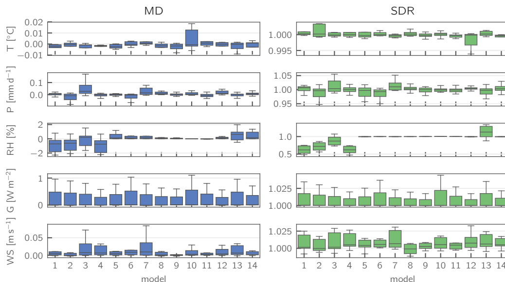
Figure 5. Mean deviation (MD) and standard deviation ratio (SDR) of simulated (i. e., downscaled and bias-corrected RCM data) vs. observed meteorological data for the historical period 1971–2005. The individual boxes represent the downscaled station meteorology for a given GCM/RCM combination (model IDs correspond to the ones in Table 2). Units given for the different variables apply only to MD (SDR is unitless).
