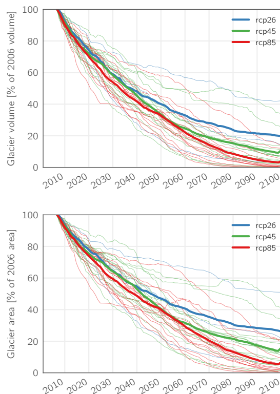
Figure 11. Simulated total glacier volume (top) and area (bottom, both shown as changes relative to the year 2006) for all glaciers in the study area and all 31 available climate scenarios. Thin lines indicate individual model results, thick lines show the multi-model mean. The small spikes in the multi-model means for RCP4.5 and RCP8.5 at the very end of the century are due to the fact that three models could only be run until 2098.
