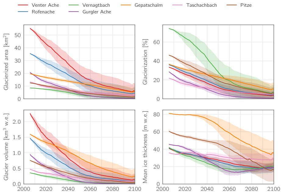
Figure 13. Evolution of the absolute (top left) and relative (top right) glacierized area for each catchment in the RCP4.5 scenario, as well as the absolute glacier volume (bottom left) and the mean ice thickness (bottom right). Note that the latter is calculated only over the glacierized fraction of the catchment and not the entire catchment area (i. e., it is the result of dividing the bottom left plot by the top left plot). Lines and shadings represent multi-model means \pm one standard deviation.
