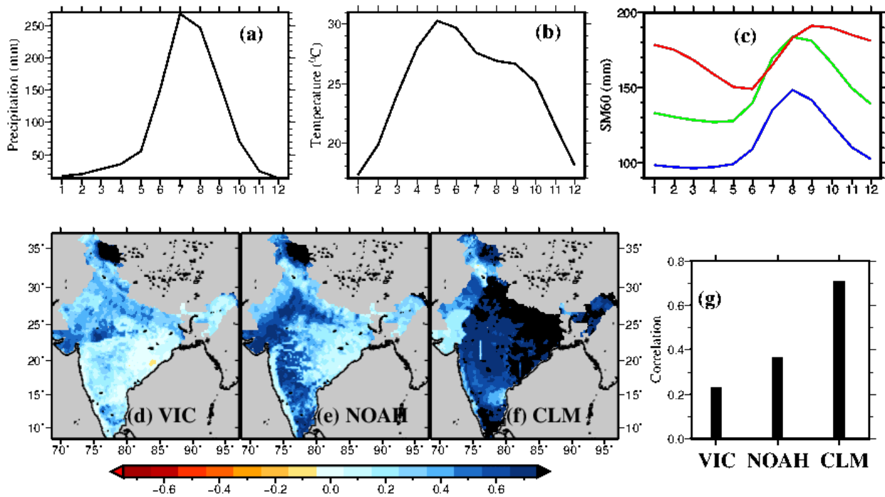
Figure 3: Uncertainty in persistence in root-zone soil moisture (60 cm). Seasonal cycle of all-India averaged (a) precipitation (b) mean air temperature and (c) 60 cm soil moisture simulated using the VIC (blue), the Noah (green), and the CLM (red). (d,e,f) Autocorrelation in 60 cm soil moisture at 4-month lag simulated using the VIC, Noah, and CLM, respectively. (g) All-India median autocorrelation in the 60 cm soil moisture from the three LSMs.
