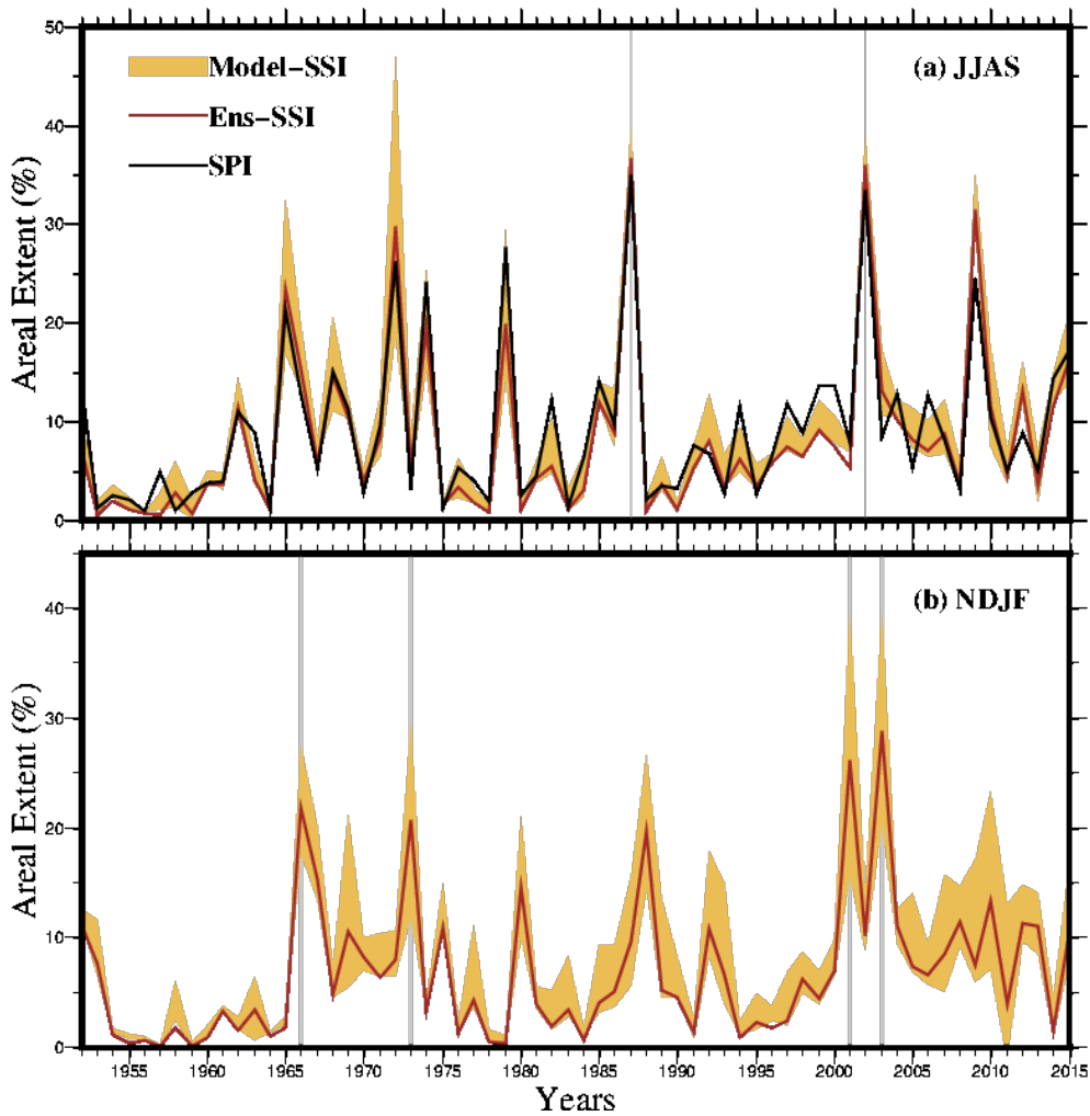
Figure 2: Uncertainty in areal extent (%) of 60 cm soil moisture drought simulated using the three LSMs (i.e. VIC, Noah, and CLM). (a) Multimodel ensemble (brown) mean 4-month Standardized Soil Moisture Index (SSI) and inter-model variation (shaded) estimated as one standard deviation for the monsoon season. Black line in (a) shows 4-month Standardized Precipitation Index (SPI) at the end of the monsoon season (June through September) (b) multimodel ensemble mean and uncertainty in 4-month SSI estimated using the three LSMs for the Rabi season (November through February). Light brown shaded area shows uncertainty in severe-to-exceptional drought based on model simulated SSI (SSI < -1.3). Dark brown line shows areal extent estimated based on ensemble mean SSI for the three LSMs. Grey line marks top drought years based on area under drought.
