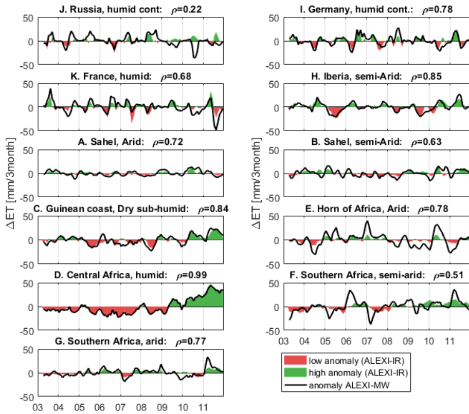
Figure 7: Comparison of anomaly in 3-month ET totals as calculated from ALEXI-IR and ALEXI-MW for selected regions (see Fig. 3 for definition of regions).
