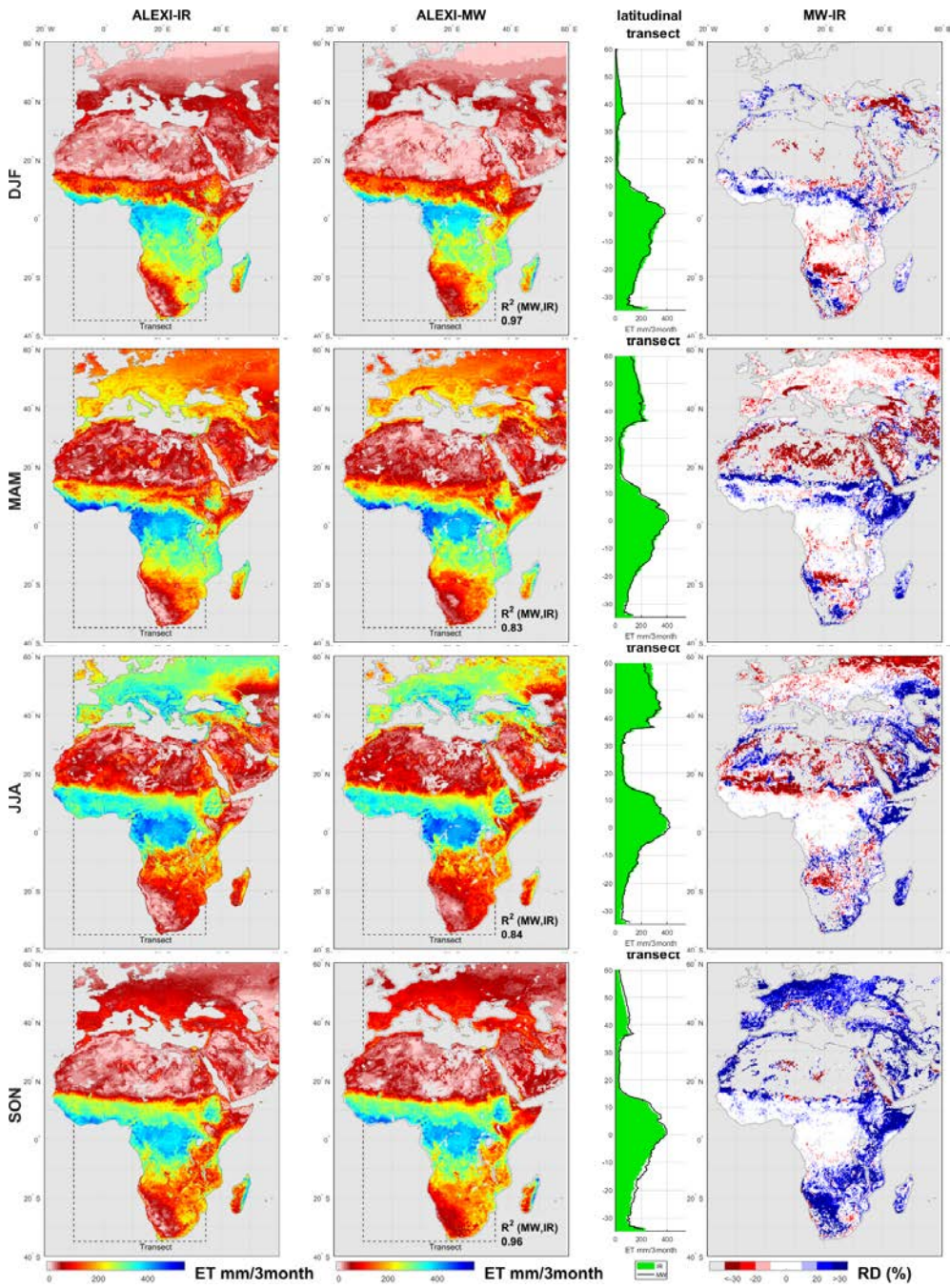
Figure 6: As Fig 4, but now averaged by season.
