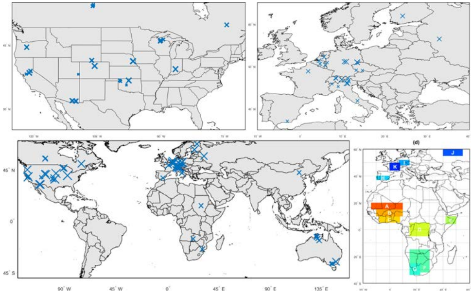
Figure 3: Location of flux tower sites used in the analysis (see also Table 2): (a) North America, (b) Europe, (c) World. The size of the marker is in proportion to number of data days used in assessment. Panel (d) indicates the 11 regions selected based on annual precipitation cycle and geographic diversity.
