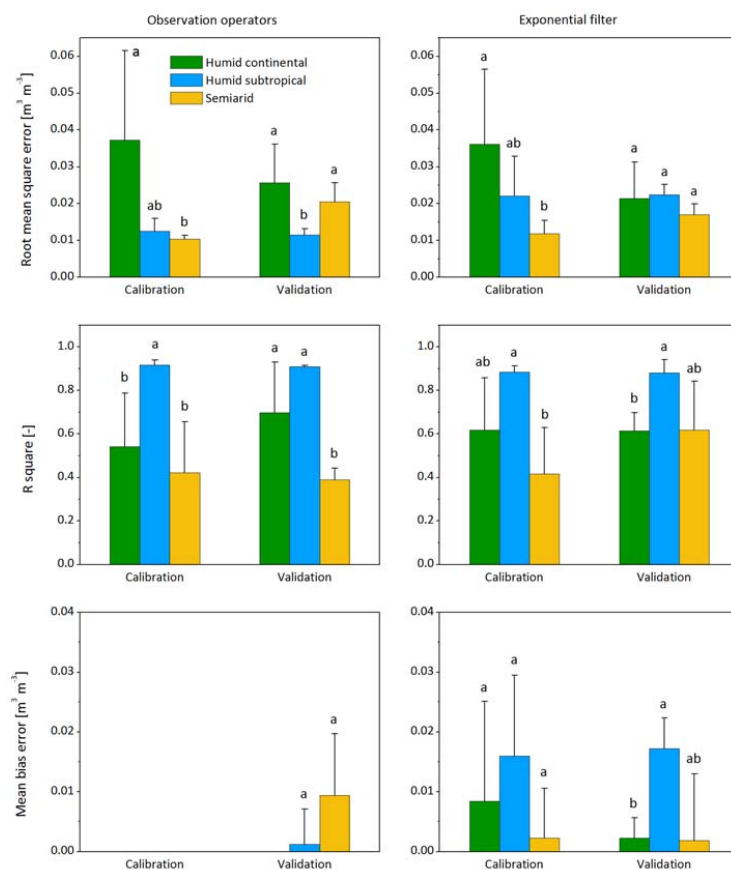
Figure 9. Statistics of the root mean square error (RMSE), R^2 and mean bias error (MBE) for the performance of observation operators and exponential filter methods in the different sites in humid continental, humid subtropical and semi-arid climates. Different lowercase letters above bars indicate significant ( P < 0.05 ) differences between climates in either calibration or validation period.
