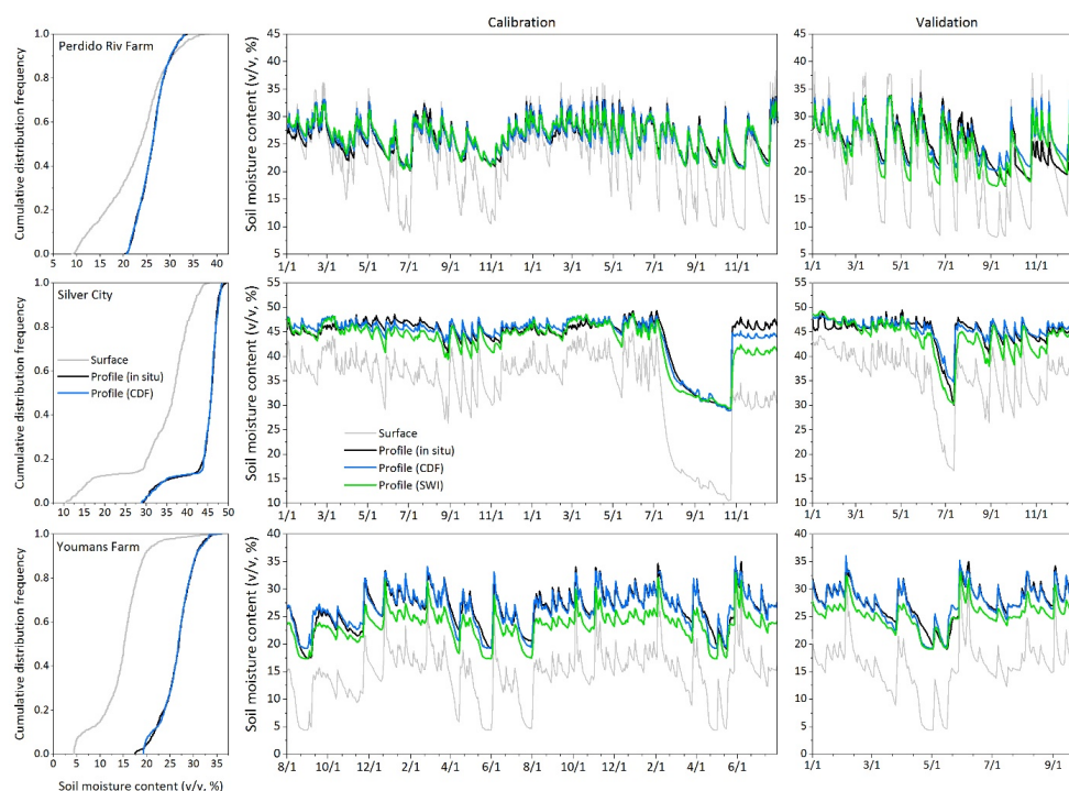
5 Figure 7. The predicted profile soil moisture by cumulative distribution frequency (CDF) matching (Profile (CDF)) and exponential filter (Profile (SWI)) during calibration and validation periods for the three sites in humid subtropical climate. The three graphs in the left shows the CDFs of surface and measured and predicted profile soil moisture.
