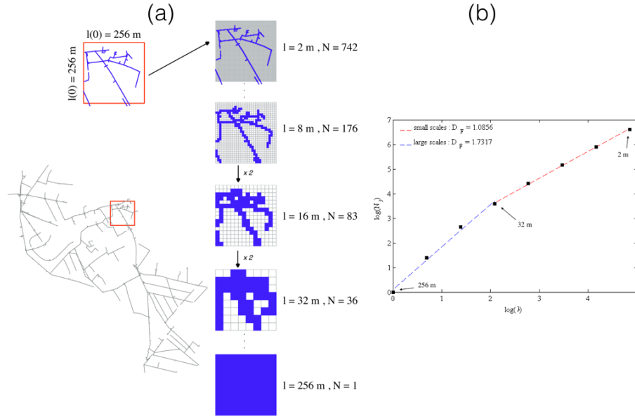
Figure 7. Example of Fractal analysis of a portion of the sewer network (256 m size) (a) N_\lambda is plotted as function of \lambda in a log-log plot (b) A scaling behaviour is retrieved over two separate ranges of scales with a break around 32 m
