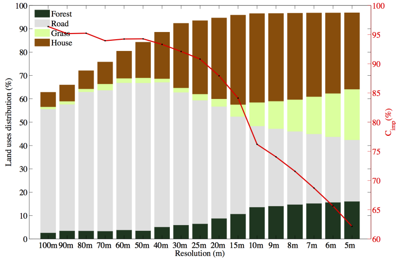
Figure 12. Scale dependency observed in the overall distribution of land cover classes and the imperviousness coefficient C_{imp} with priority rule as explained in Figure 2. The priority order was set up as follows: gully, road, forest, house, grass.
