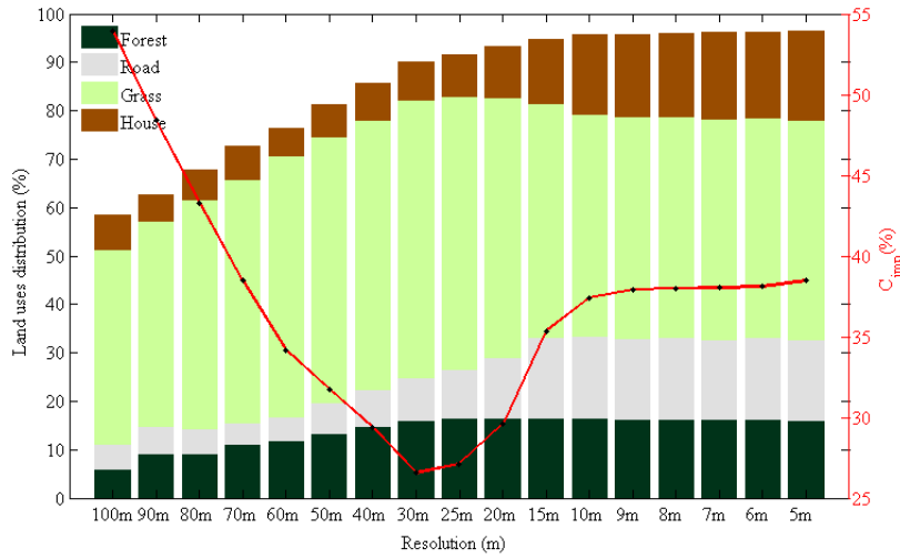
Figure 13. Scale dependency observed in the overall distribution of land cover classes and the imperviousness coefficient C_{imp} with majority rule as explained in Figure 2
