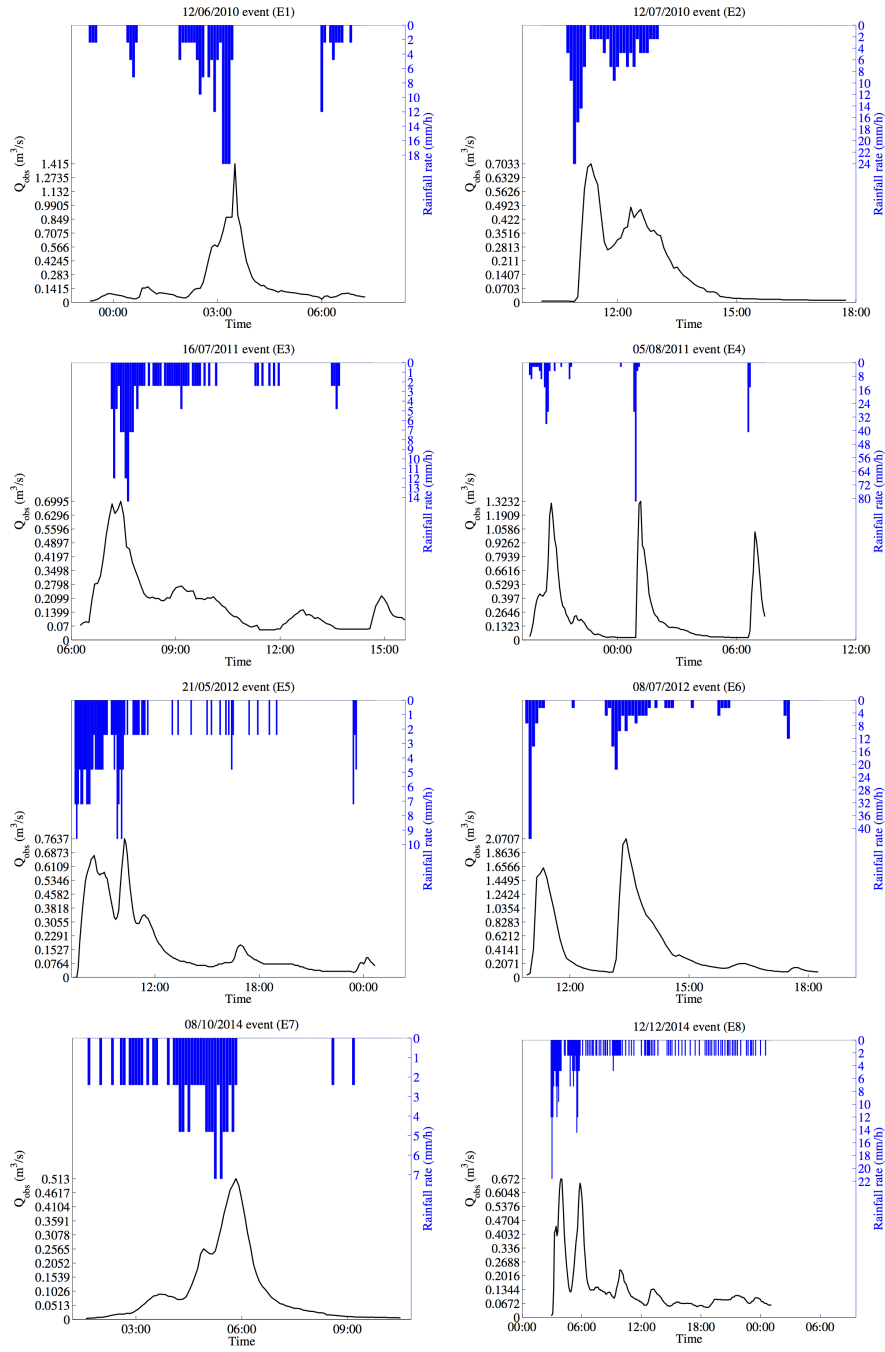
Figure 6. Rainfall data and the corresponding flow measurement available for the 8 rainfall events selected to perform the multi-scale modelling investigation.
