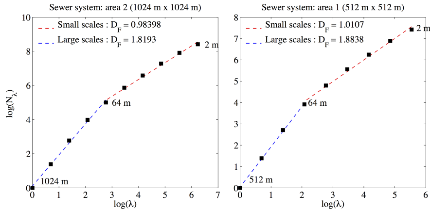
Figure 10. Fractal analysis of the sewer system structure. Two ranges of scale are identified on both areas; D_f is equal to 1 at small scales (2 m-64 m) and 1.8 for large scales l \geq 64 m
