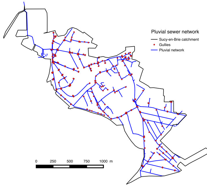
Figure 5. The storm water system of Sucy-en-Brie catchment which is used to implement Multi-Hydro model
