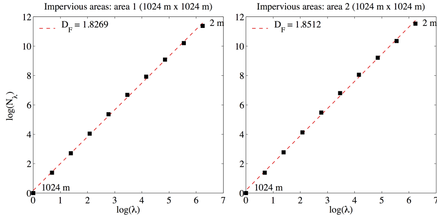
Figure 11. Fractal analysis of the impervious data. One unique scaling regime is identified across the whole range of available scales (2 m-1024 m); D_f is greater than 1.8 for both areas.
