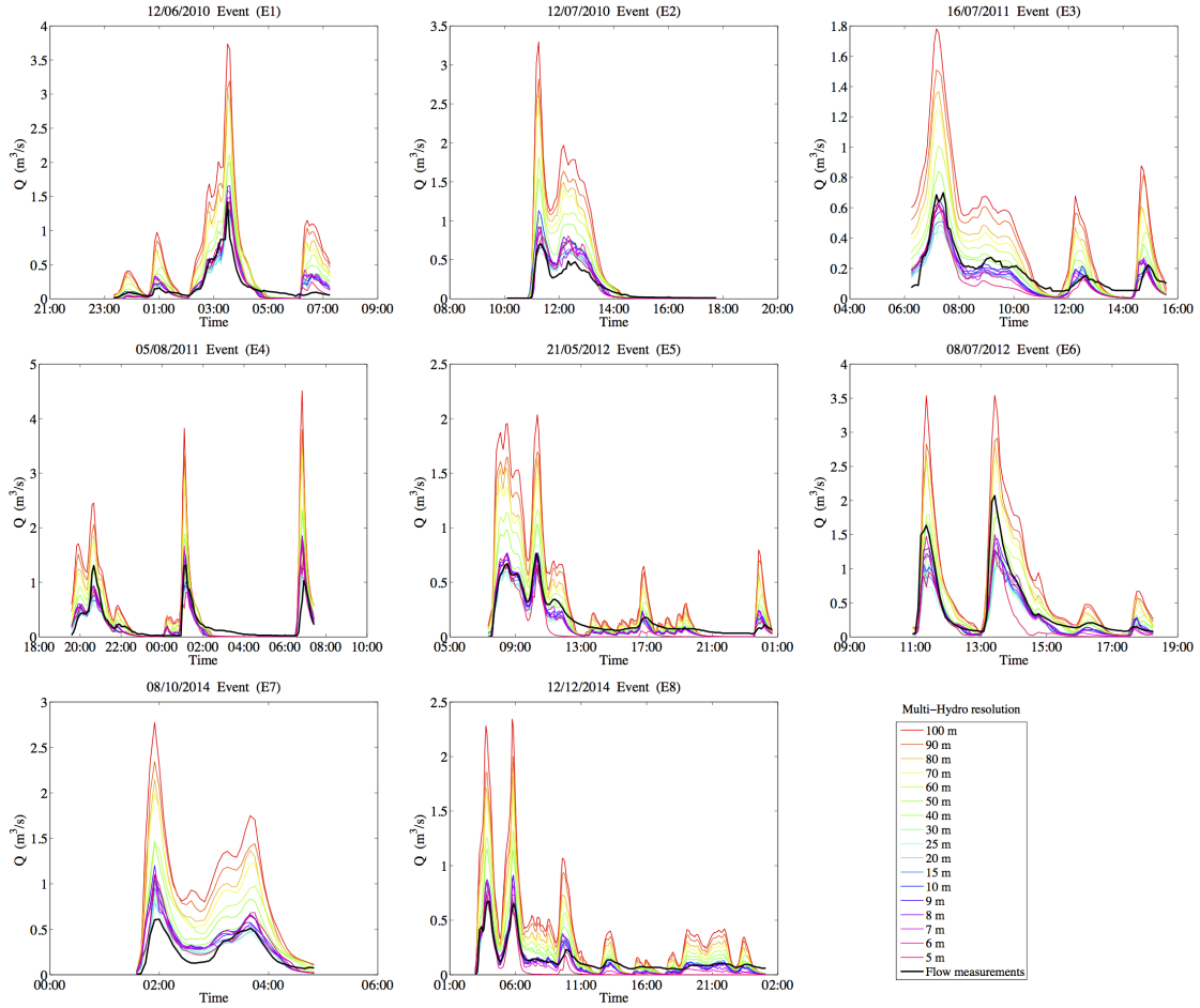
Figure 14. Multi-scale modelling outputs compared with observed flow, one can notice the high sensitivity of Multi-Hydro response to the spatial resolution of the model
