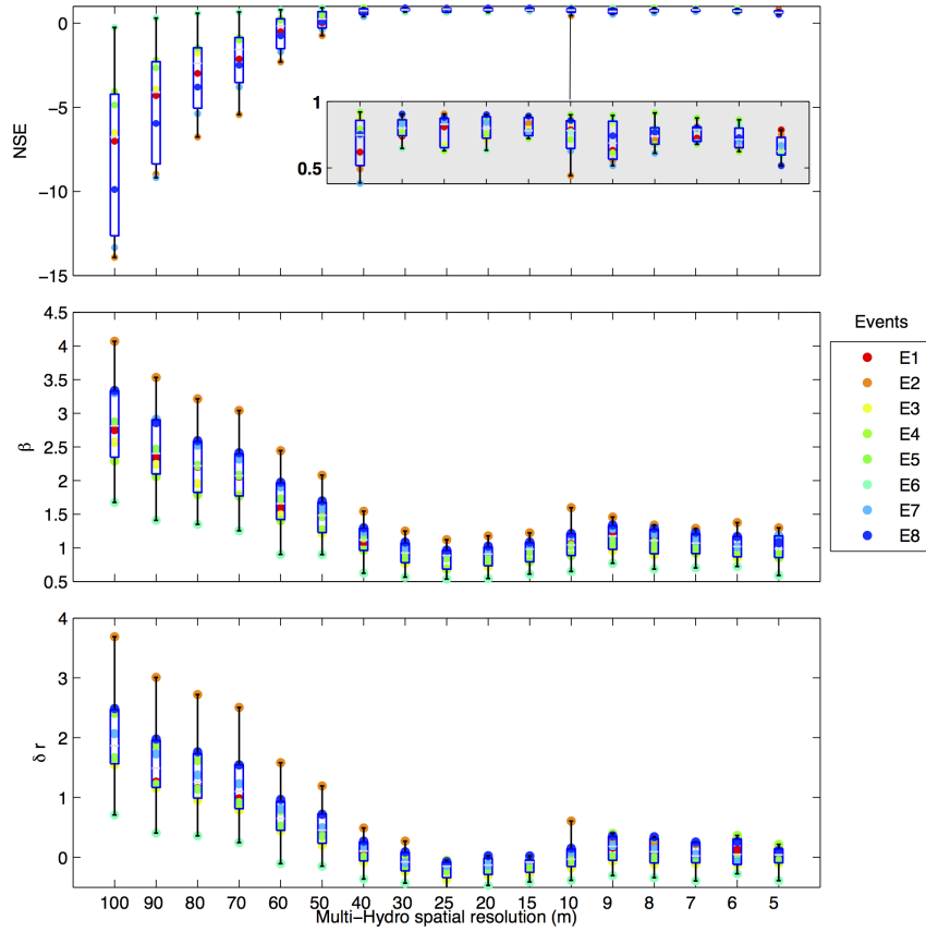
Figure 16. Performance indicators NSE , \beta and \delta r estimated from Multi-Hydro modelling outputs obtained at the 17 spatial scales with respect to observed data.
