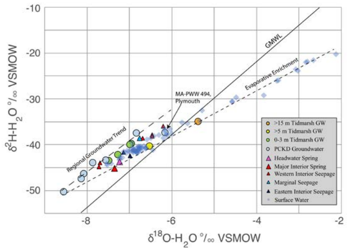
Figure 8: Plot of the stable isotopes \delta^2\text{H-H}_2\text{O} and \delta^{18}\text{O-H}_2\text{O} from the Tidmarsh Farms area surface water (diamonds), groundwater (circles), shallow well, and seep sources (triangles). The regional groundwater trend line was derived from samples from relatively shallow, regional USGS wells (blue dots, shaded grey region), consistent with a relatively humid climate at the site.
