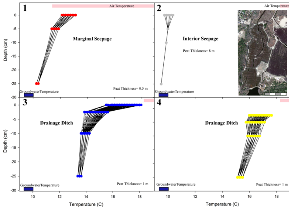
960 Figure 7: Temperature profiles vs. depth at Tidmarsh Farms recorded in July 30-31, 2013. For each profile, the range of air temperatures and groundwater (GW) temperatures are shown as bands of pink (air) and dark blue (groundwater) bands . At the locations 1 and 2 , (profiles 1 and 2) show the influence of upwelling 965 groundwater; expressed as type 1 preferential flow path (PFP) seepage (profile 2) and type 2 matrix seepage (profile 1). The concave upward shape of temperature-depth profiles 3 and 4 is also indicative of consistent with upwelling seepage.
