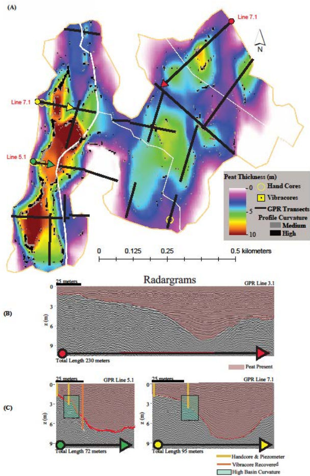
915 Figure 2: a) Map of total peat thickness beneath Tidmarsh Farms based on GPR data. GPR data collected along 920 linear transects shown here (black lines; pink lines on Figure 1B) were interpolated and contoured to show peat thickness (colors) on the 2D surface map. Zones of medium and high curvature (the 2nd derivative of the thickness) of the peat-sand interface are shown as grey and black pixels, respectively. b) and c) Three example cross sectional profiles, or radargrams, illustrate a distinct reflector at the basal peat-sand contact. Peat is shaded red, and sediment cores samples used to constrain the GPR velocity data are also shown as yellow lines (hand cores) and orange lines (vibracore) were used to constrain the GPR velocity data. High curvature is highlighted in green boxes.
