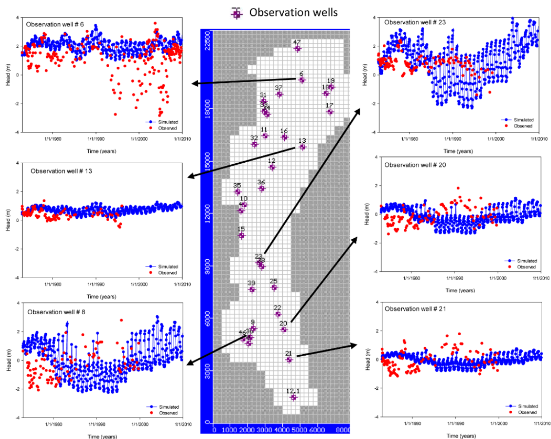
Figure 11.a: Hydraulic head obtained with the models vs. data at some observation points.
