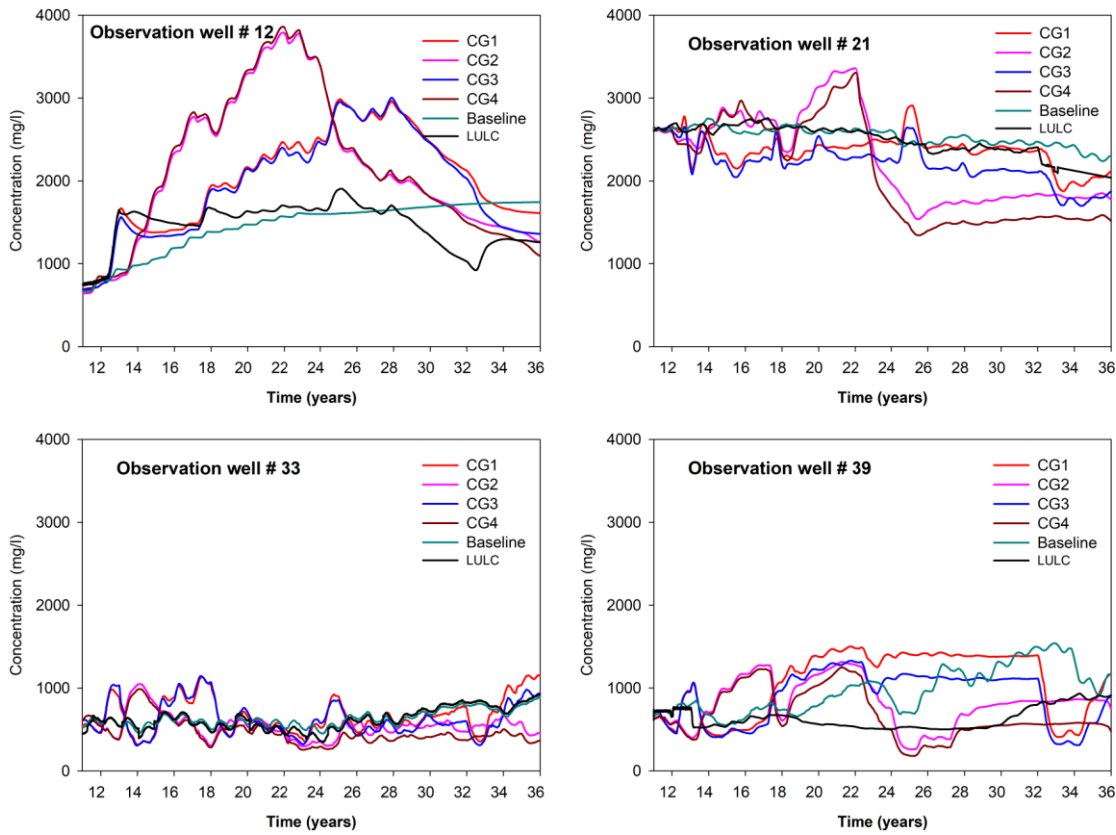
Figure 14: Evolution of future salinity concentration at four observation points for the Baseline (BL) scenario and the four Global Change scenarios.
