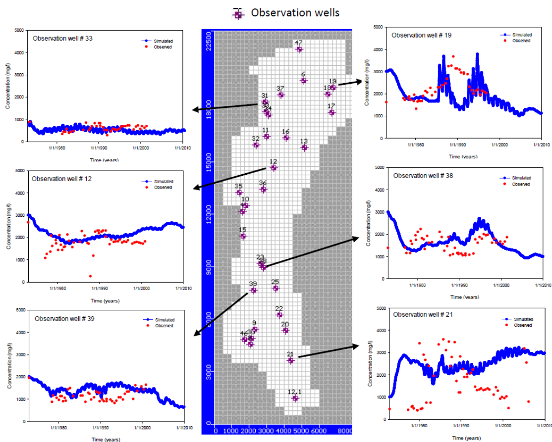
Figure 11.b: Salinity obtained with the models vs. data at some observation points.
