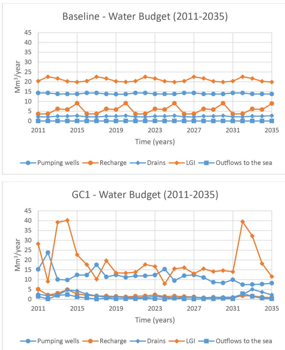
Figure 12: Components of the flow budget evolution for the BL scenario and the mean of the potential future GC1 scenarios (horizon 2011-2035).
