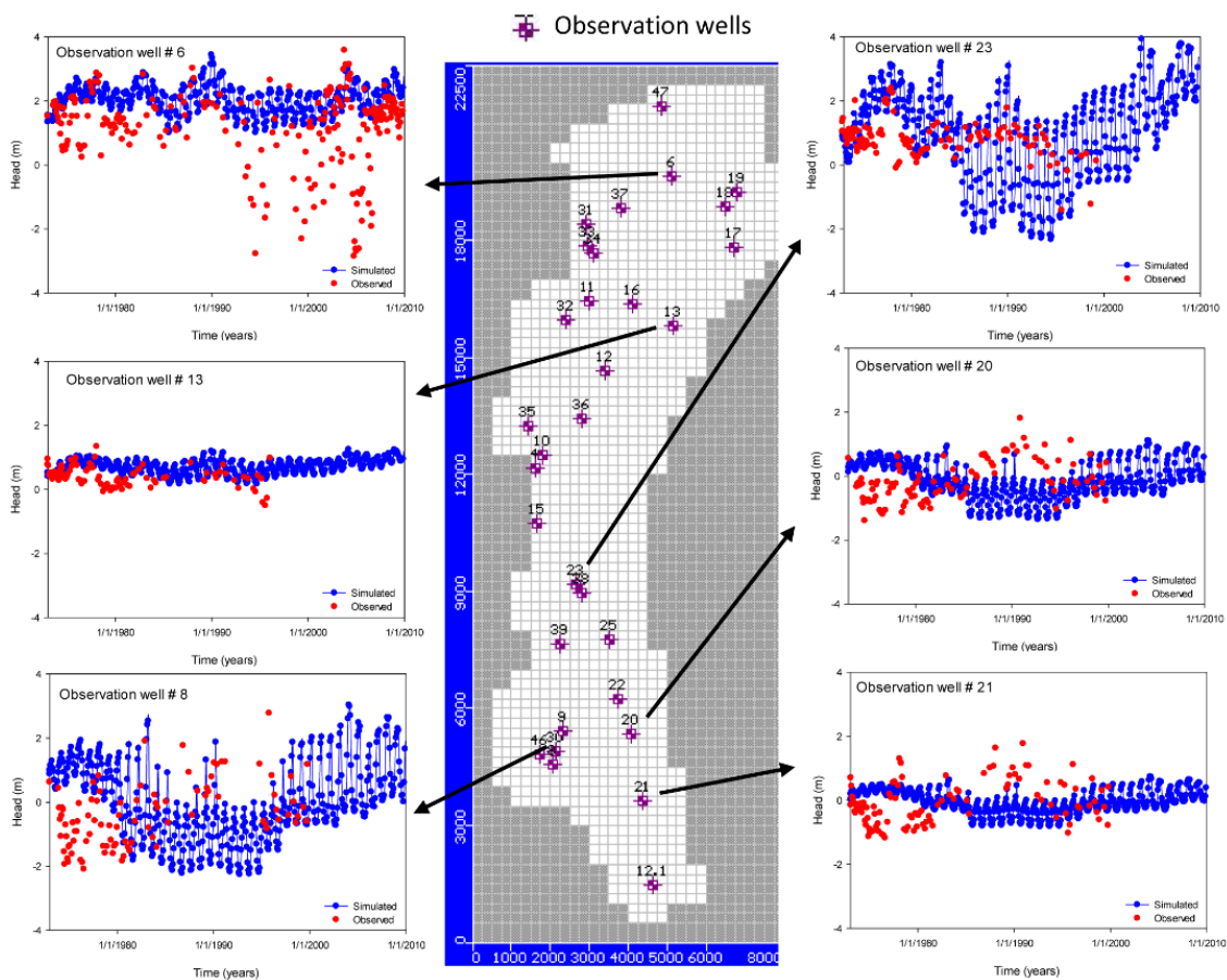
Figure 11.a: Hydraulic head obtained with the models vs. data at some observation points.
