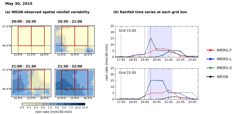
Figure 7. Example rainfall event in the warm season that occurred on 30 May 2015. (left) Spatial rainfall pattern over the WEGN network area for a sequence of four consecutive half-hourly WEGN rain rate maps, with periods over the two selected IMERG grid cells indicated (red-framed boxes (red outline; see Fig. 1). (right) Time series of IMERG-F (red), IMERG-L (blue), IMERG-E (green) estimates and WEGN (black) data for the two IMERG in each grid cells over the period of box during the rainfall event, with the shaded areas highlighting the two hours illustrated by the map sequence to the left in (a). Solid vertical lines indicate time steps where all three IMERG runs received PMW-based information for the rainfall retrieval at that time step, dotted vertical lines (not applicable for this event but for the event of Fig. 8 below) mean that either IMERG-E or both IMERG NRT runs did not receive PMW-based information at the time step, and no vertical line (the case for most time steps) implies that none of the IMERG runs received PMW-based information.
