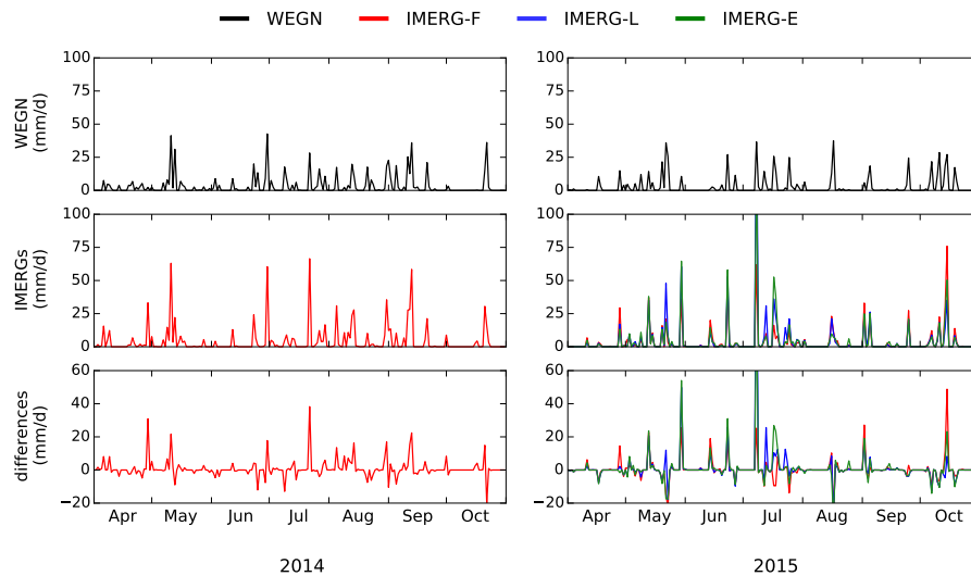
Figure 3. Accumulated 24-h rainfall (mm/d) over the selected study periods in 2014 (left) and 2015 (right), obtained from WEGN data (top) and IMERG estimates runs (middle), and differences of the between IMERG estimates against and WEGN data (bottom). Regarding IMERG ; in the 2014 period, only IMERG-F data are available.
