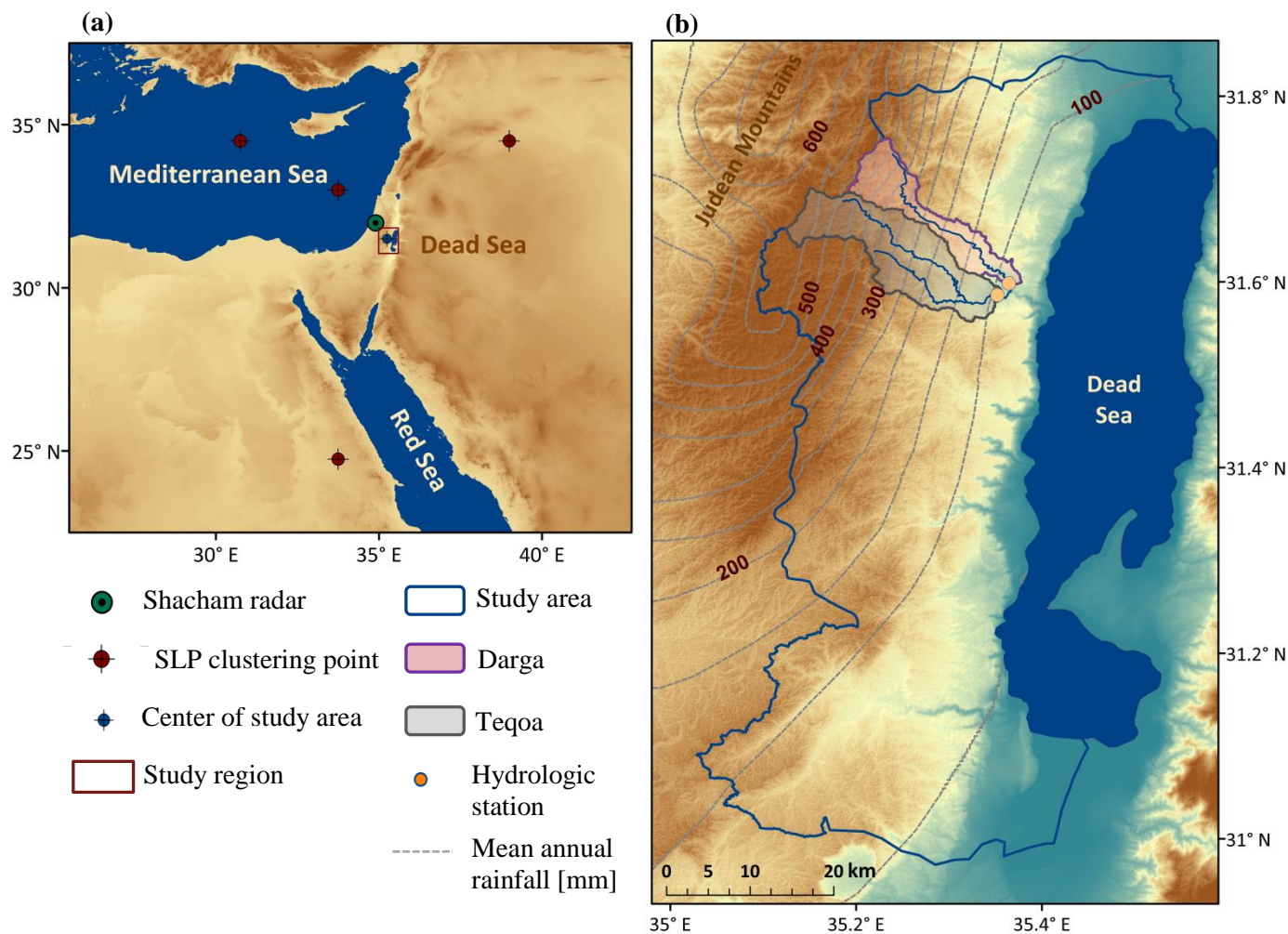
Figure 1: Map of the Eastern Mediterranean area presenting radar location and coordinates used to derive SLP differences for synoptic classification (a). A map of the study area with the Darga and Teqoa catchments (b). Isohyets over the study region represent long-term (30 years, 1980-2010) mean annual rainfall [mm].
