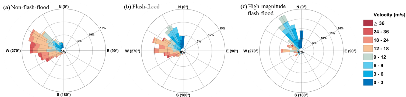
Figure 11: Advection (velocity and direction) distributions of dominant rain cells for: (a) non-flash-flood events (490 cells, 144 events), (b) flash-flood events (220 cells, 29 events) and (c) high-magnitude flash-flood events (111 cells, 15 events). High magnitude is defined based on median values of measured flash-floods in Darga and Teqoa, used in this analysis.
