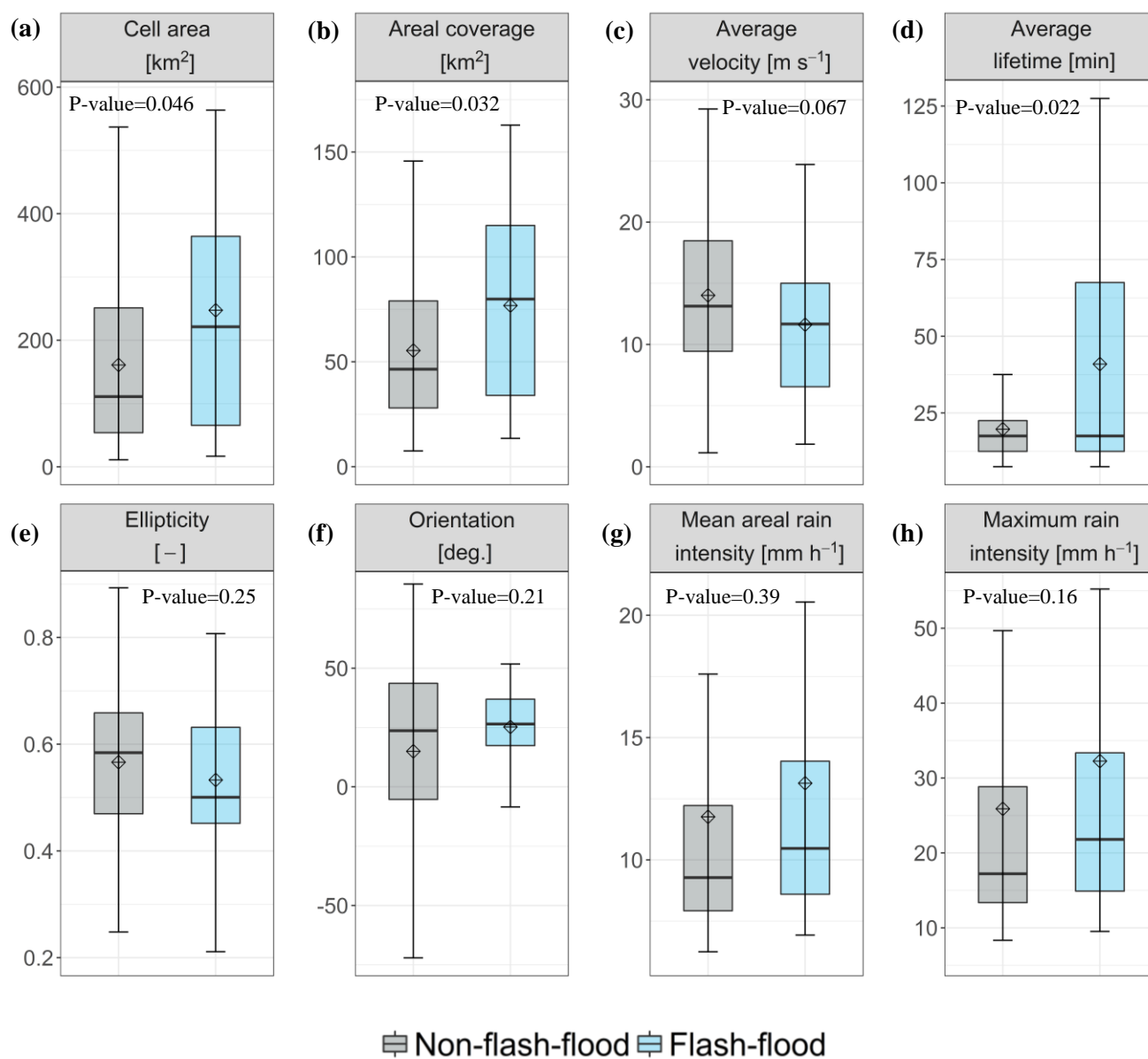
5 Figure 10: Comparison of dominant flash-flood related cells (blue, N=29) and non-flash-flood related cells (grey, N=144) properties: (a) cell area [km 2 ], (b) areal coverage [km 2 ], (c) average velocity [m s -1 ], (d) average lifetime [min], (e) ellipticity, (f) orientation [deg.], (g) mean areal rain intensity [mm h -1 ], (h) maximum rain intensity [mm h -1 ]. Values are averaged over the dominant cell's lifetime.
