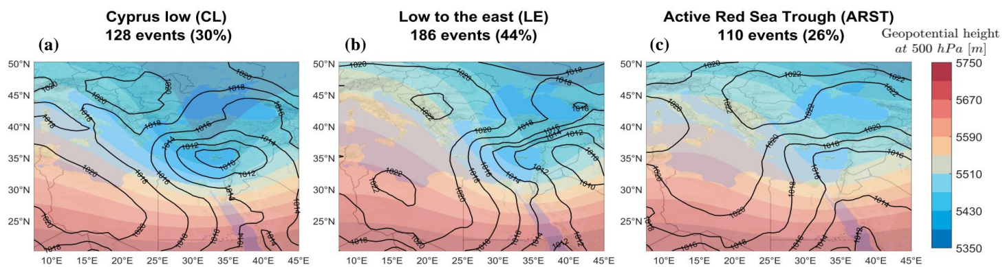
Figure 3: Average SLP [hPa] (black contour lines) and geopotential height [m] at 500 hPa (in color) for each cluster; (a) Cyprus low, (b) low to the east and (c) Active Red Sea Trough.
