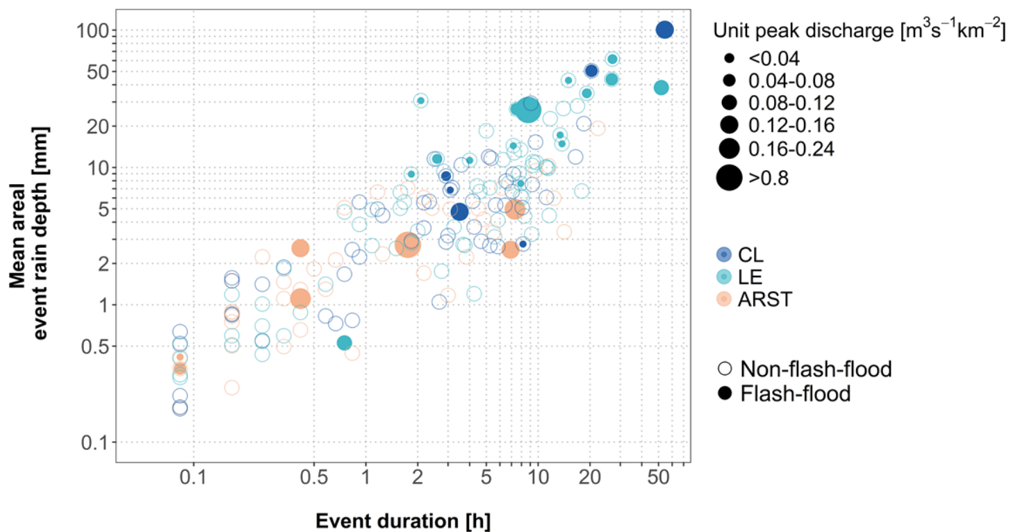
5 Figure 9: Scatter plot of rain events' mean areal rain depth over the catchments vs. duration, for flash-flood associated (filled circles) and non-flash-flood (empty circles) events, with respect to different synoptic types and different unit peak discharges of the flash-flood related events. In case of flow in both catchments, maximum unit peak discharge is presented. Event duration refers to the part of the event where rain cells were found over the catchments.
