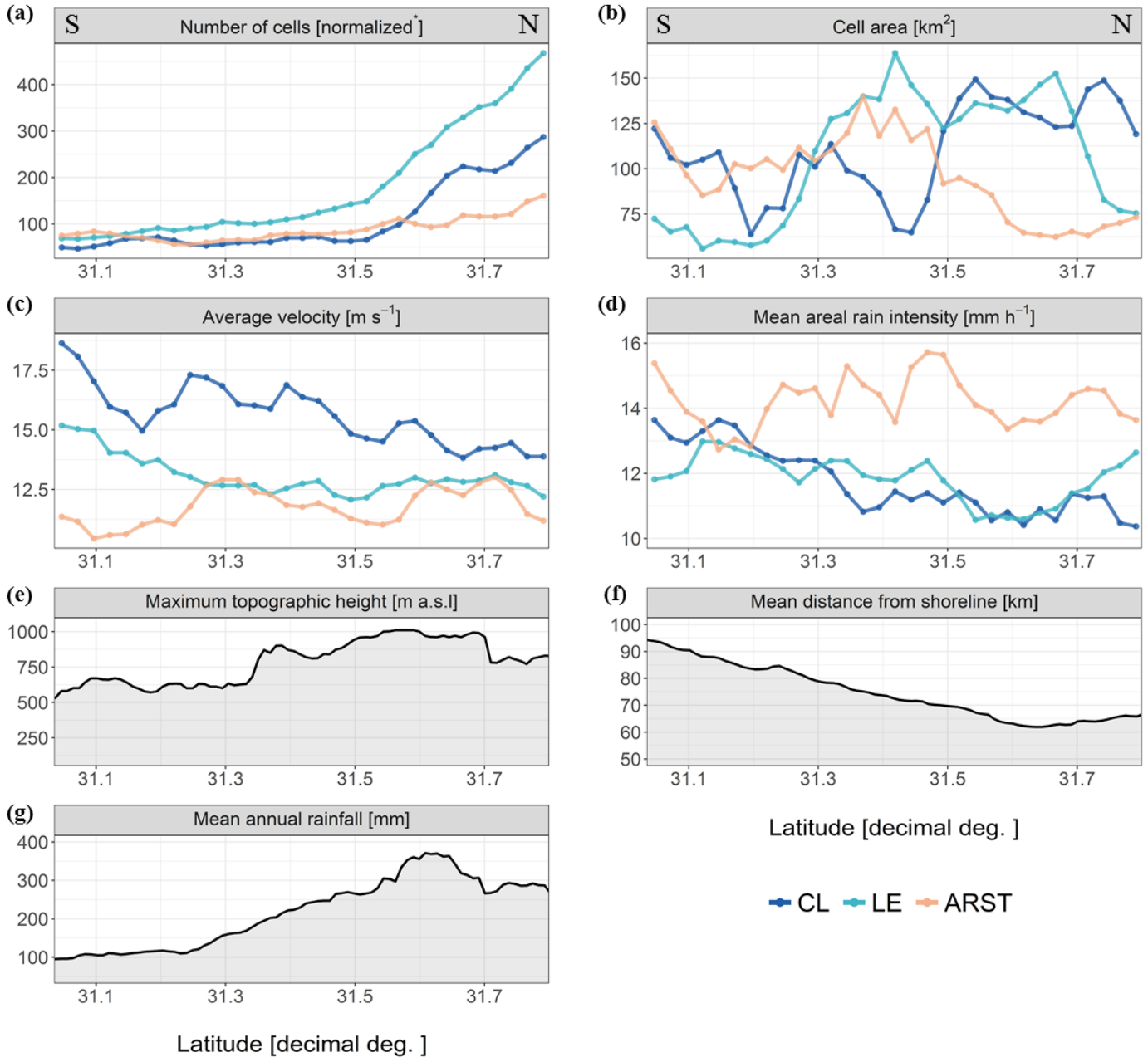
Figure 8: Mean rain cells' properties along a north (right)-south (left) axis of the different synoptic systems: (a) number of cells*, (b) cell area [km 2 ], (c) average velocity [m s -1 ], (d) mean areal rain intensity [mm h -1 ]. Potentially related variables along the same axis: (e) maximal topographic height [m a.s.l.], (f) distance from shoreline [km] and (g) mean annual rainfall [mm]. Each point represents mean or maximal value in a west to east strip (in figures a-d strip is 2.5 km wide and a running average of 7.5 km is applied). *Number of cells is normalized to the relative strip area.
