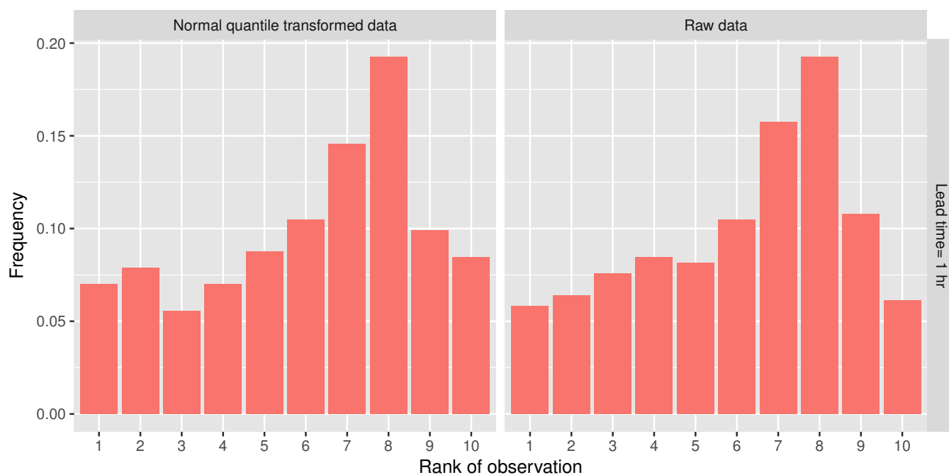
Figure 9. Rank histograms for the WRF ensemble for the Mugroso watershed for the finest domain (resolution of 1.67 km) and lead times up to 6 hours.
