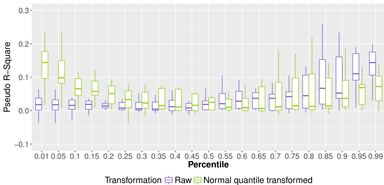
Figure 3. Pseudo R-Square for the Mugroso watershed for the coarsest domain and lead times up to 12 hours.
