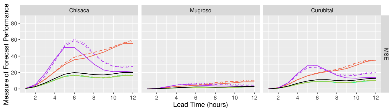
Figure 7. Performance Measures for deterministic discharge and ensemble mean forecasts obtained excluding the storm with the highest precipitation missed by the WRF model. Domain 1, domain 2 and domain 3 correspond respectively to the domains with resolutions 15 km, 5 km and 1.67 km. The legend is the same as in Figure 6.
