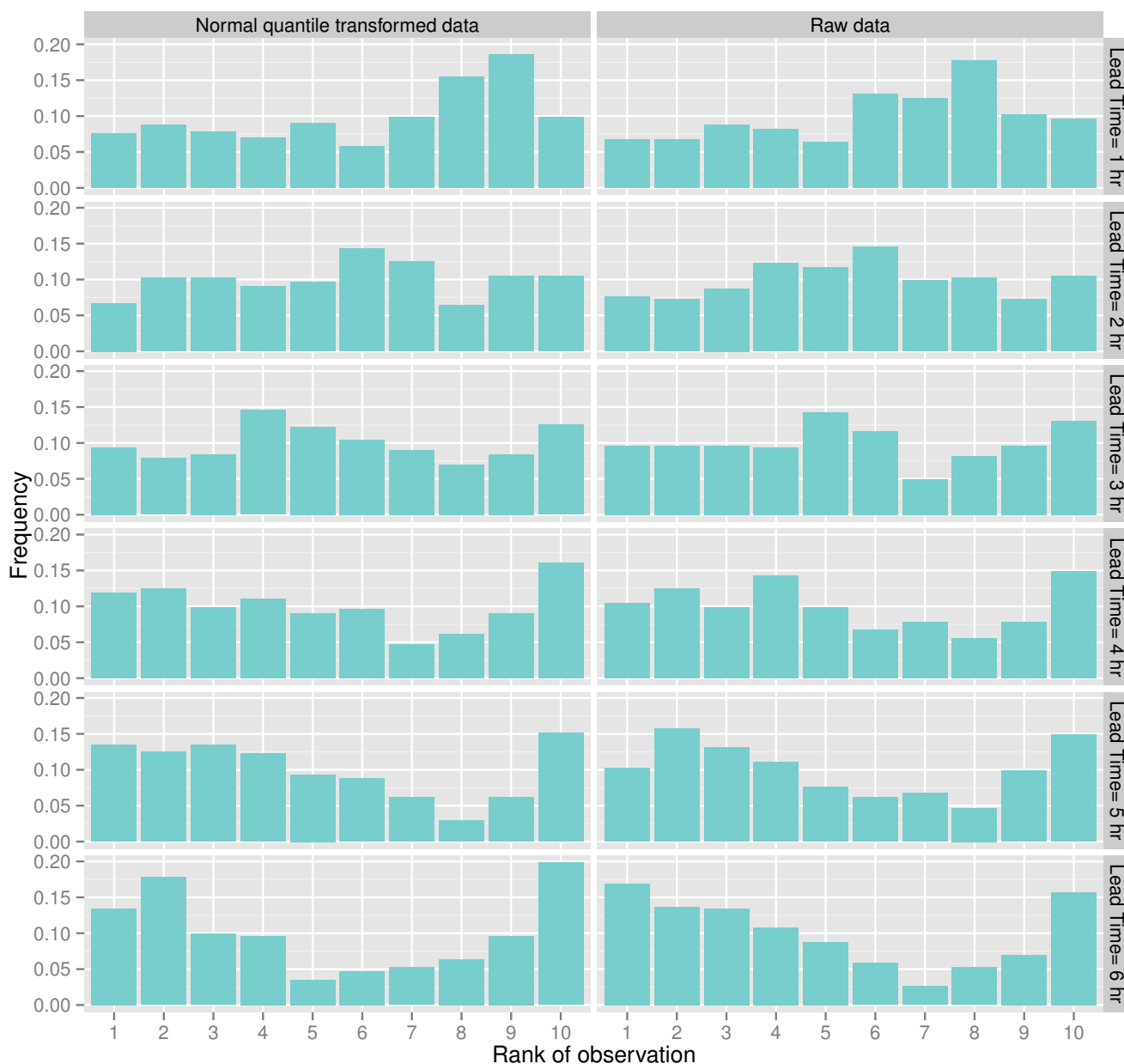
Figure 10. Rank histograms for the Q ensemble using as reference time series the discharge simulated with the TOPMODEL.
