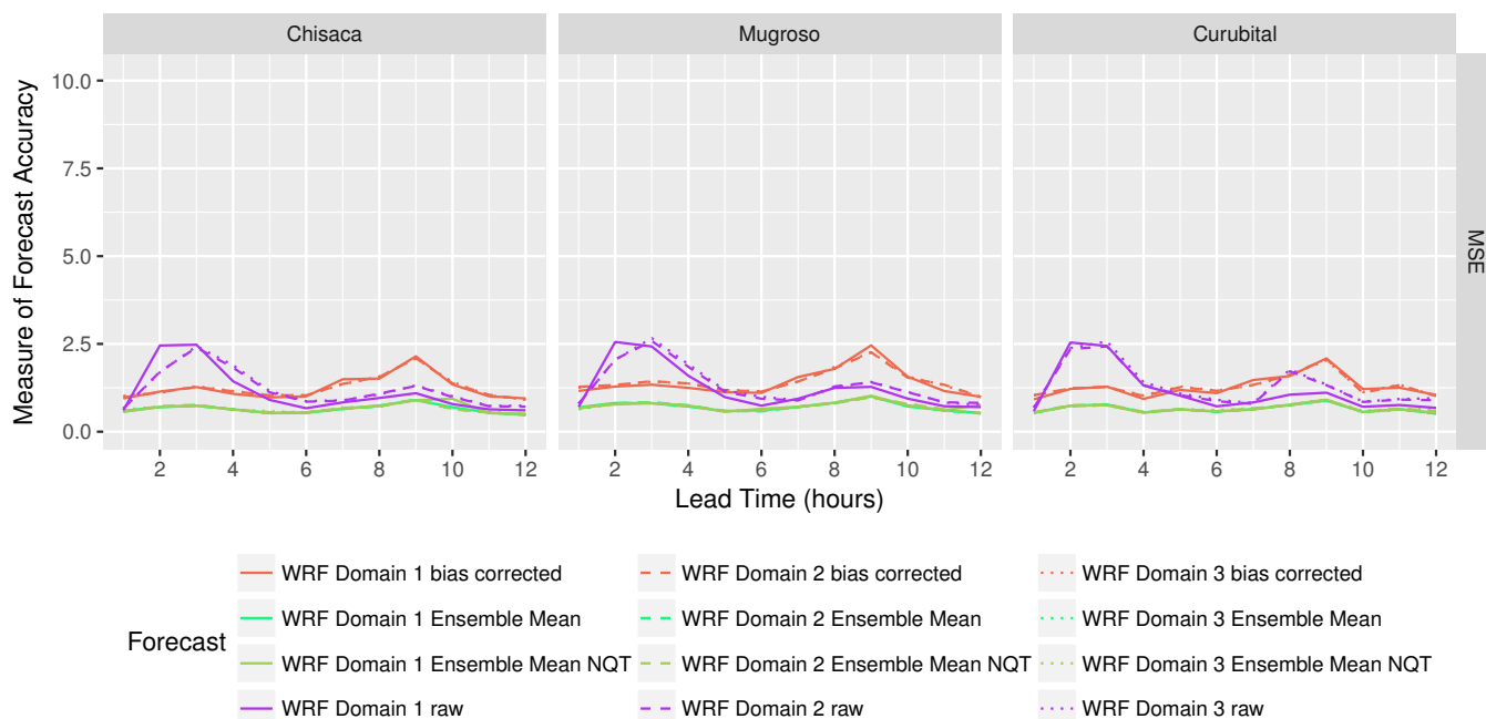
Figure 6. Accuracy Measures for deterministic precipitation and ensemble mean obtained from the WRF model without the highest precipitation missed by the WRF model. Domain 1, domain 2 and domain 3 correspond respectively to the domains with resolutions 15 km, 5 km and 1.67 km. The legend is the same as in Figure 5
