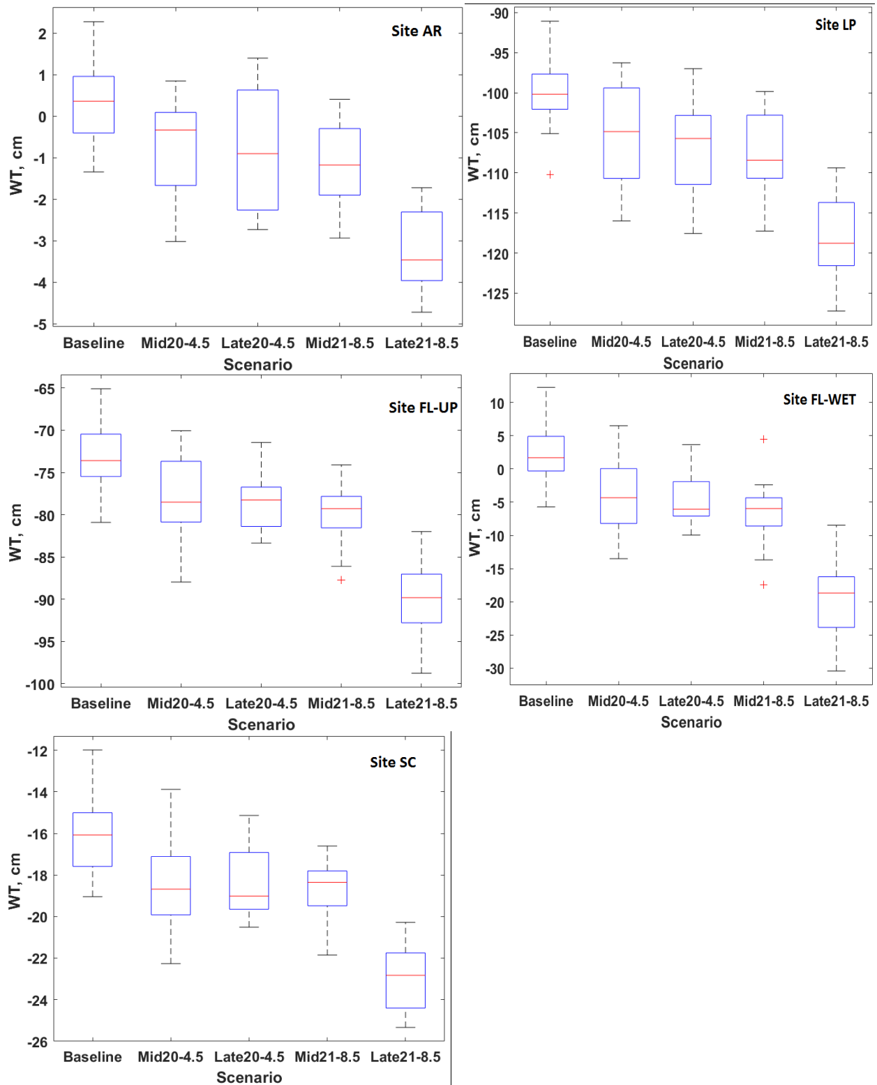
720 Fig. 5 Mean predicted annual water table of 20 GCMs in five wetlands in the southeastern United States (unit: cm).
