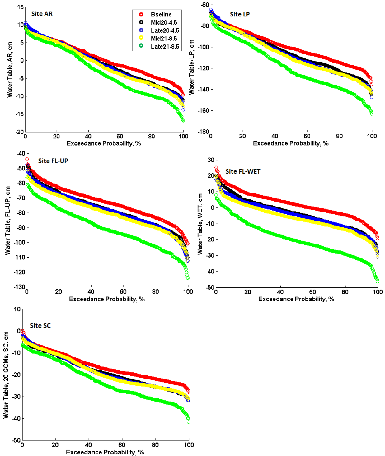
Fig. 6 Exceedance probability of the mean predicted water table in the growing season of 20 GCMs in five wetlands in the southeastern United States (unit: cm).
