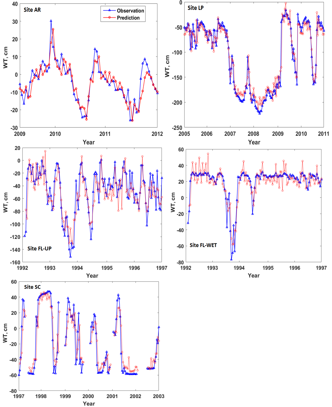
700 Fig. 2 Comparison of observed and simulated mean water table in five wetlands in the southeastern United States, WT is water table.
