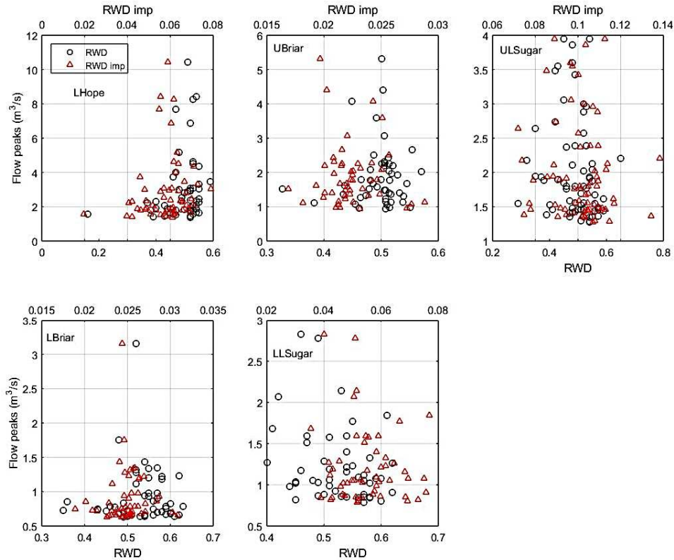
Figure 9. Scatter plots of 2h-mean RWD versus peak flow, for RWD based on all areas (lower x-axis) and for normalised RWD weighted by imperviousness (upper x-axis), for the five basins in LSugar Creek catchment.
