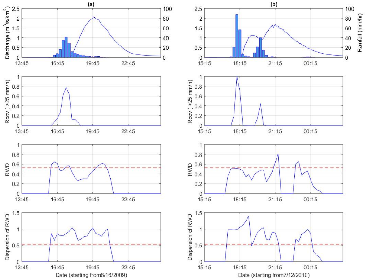
Figure 5. Time series of basin-average rainfall, flow, portion of basin covered by high-intensity rainfall ( >25 mm/h), normalised rainfall-weighted flow distance (RWD) and RWD dispersion in Lower LSugar, for 2 events that occurred on 16 August 2009 (a) and 12 July 2010 (b).
