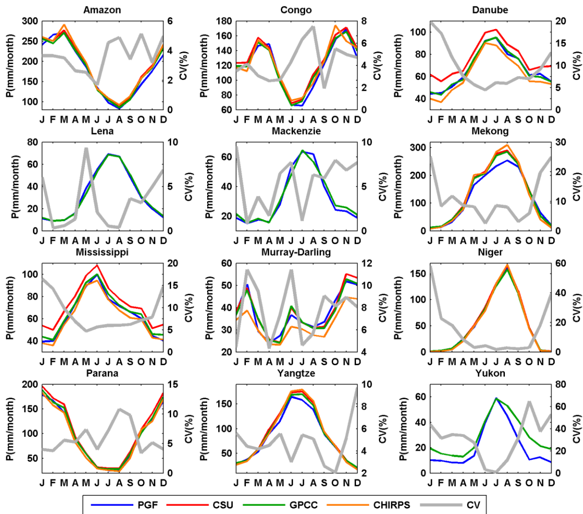
Figure 3. Seasonal cycles of precipitation from different products over twelve representative large basins for 1998-2010
