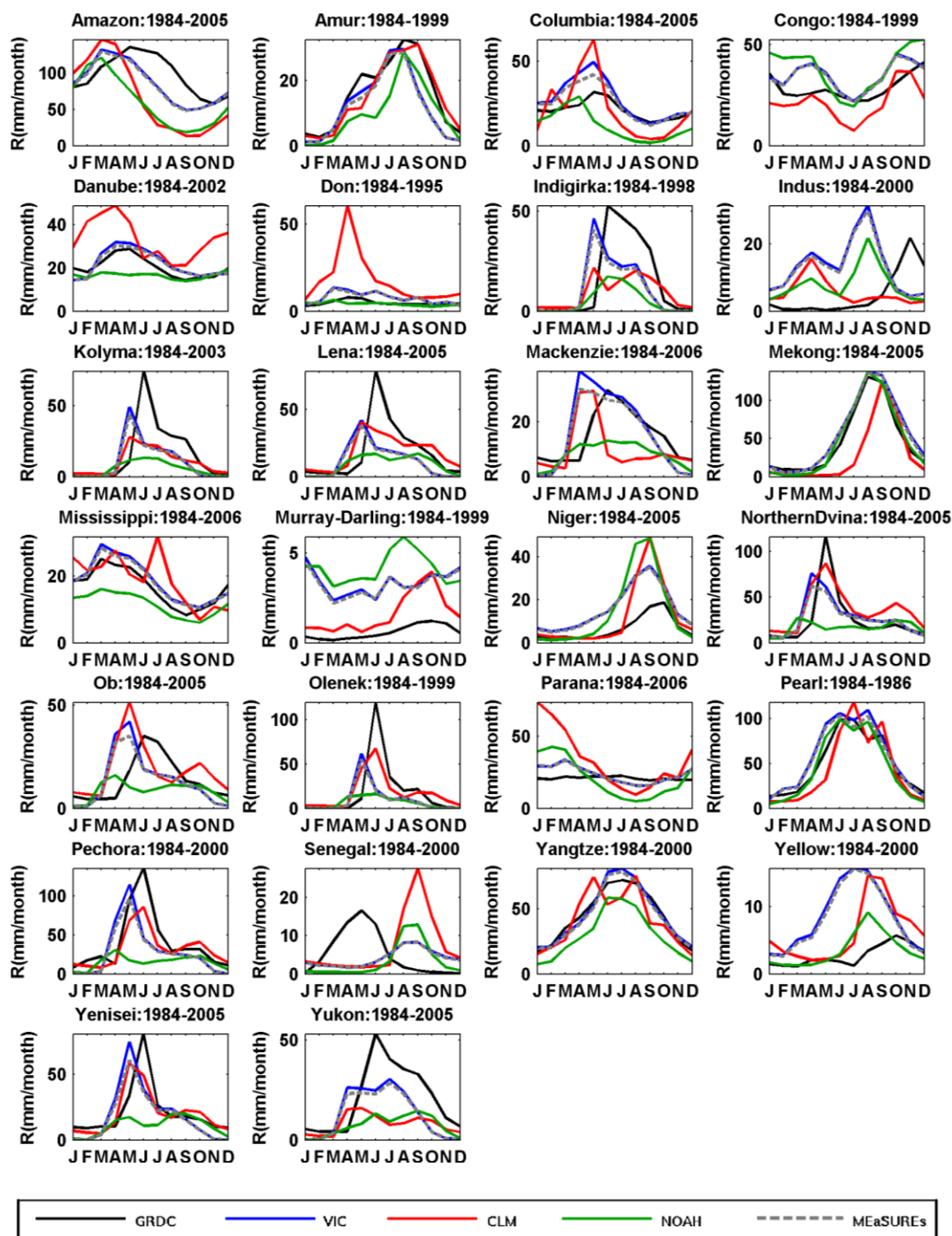
Figure 13 Seasonal Cycles of runoff from VIC, CLM, NOAH and MEaSUREs against GRDC runoff observation over 26 large basins for different periods according to in situ data availability
