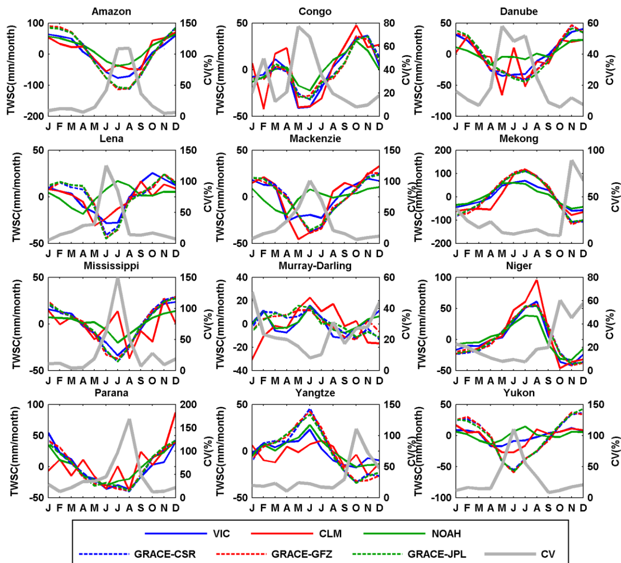
Figure 9. Seasonal cycle of total water storage change (TWSC) from different products over twelve representative large basins for 2003-2010
