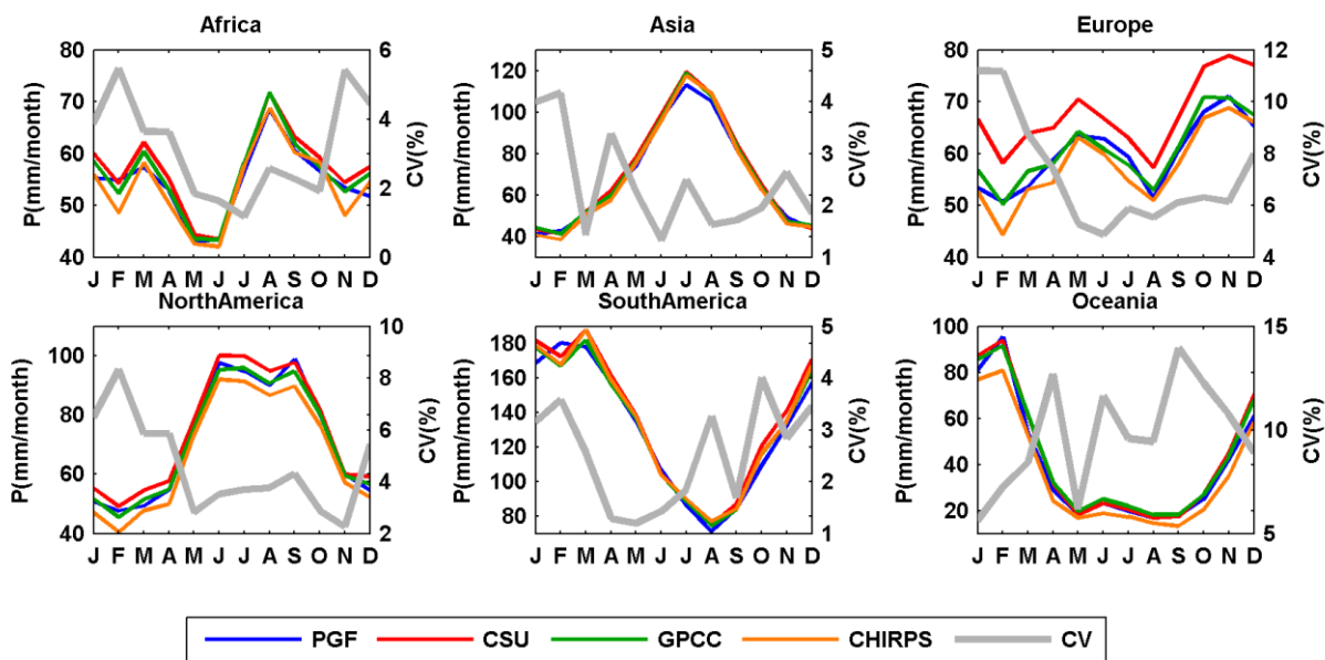
Figure 2. Seasonal cycles of precipitation from different products over the six continents for 1998-2010
