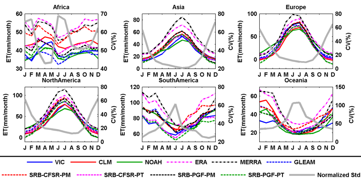
Figure 4. Seasonal cycles of evapotranspiration from different products over the six continents for 1984-2007
