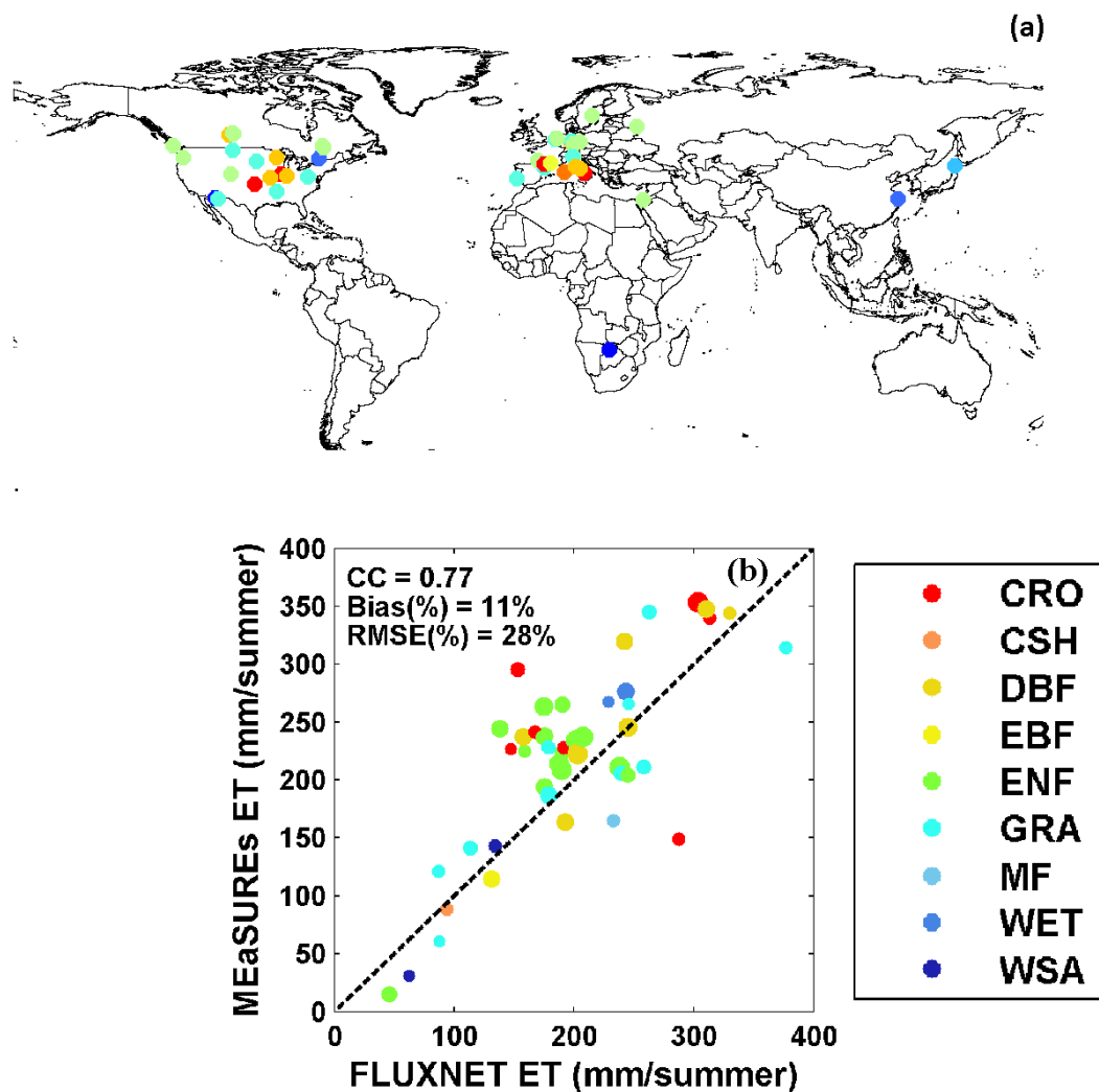
Figure 16. (a) Distributions of 47 flux towers over the globe (b) Validation of MEaSUREs ET estimates against FLUXNET observations
