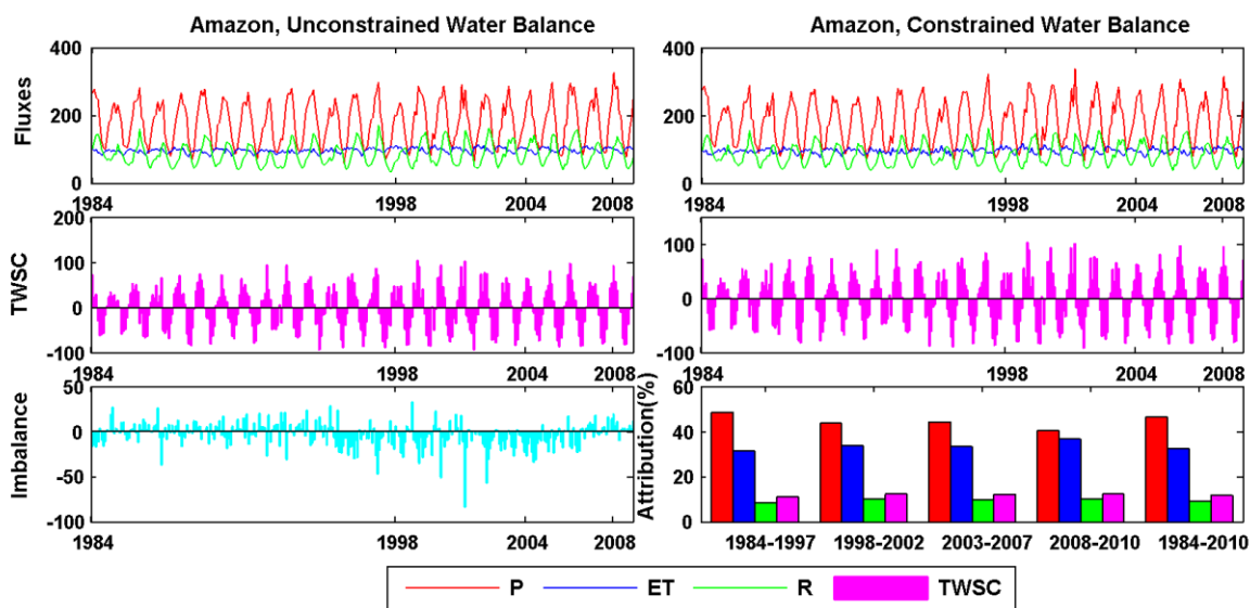
5 Figure 12. Unconstrained (left column) and constrained (right column) water budget estimates (mm/month) over Amazon River basin. The top, middle and bottom rows show the time series of water budget in terms of fluxes (precipitation, evapotranspiration and runoff), TWSC (Total Water Storage Change) and Imbalance. The imbalance/non-closure error after water budget constraint equals to zero and the imbalance/non-closure attributions to each water budget variables throughout different sub-periods are shown at the right bottom.
