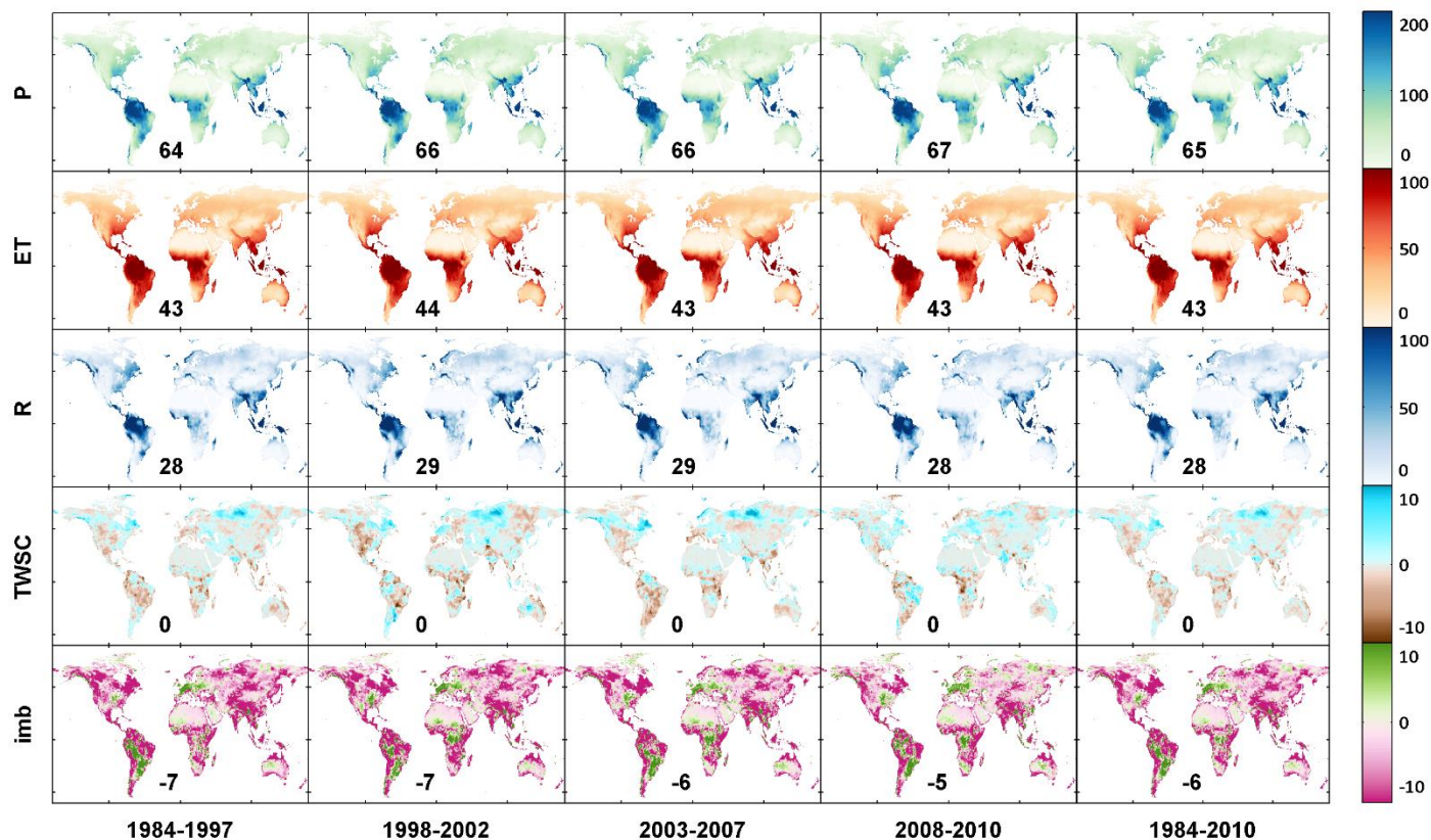
Figure 11. Monthly mean (mm/month) of different water budget terms (from the first row to the bottom: precipitation, evapotranspiration, runoff, total water storage change, imbalance) before water balance constraint throughout different periods (from the left to the right: 1984-1997, 1998-2002, 2003-2007, 2008-2010, and 1984-2010)
