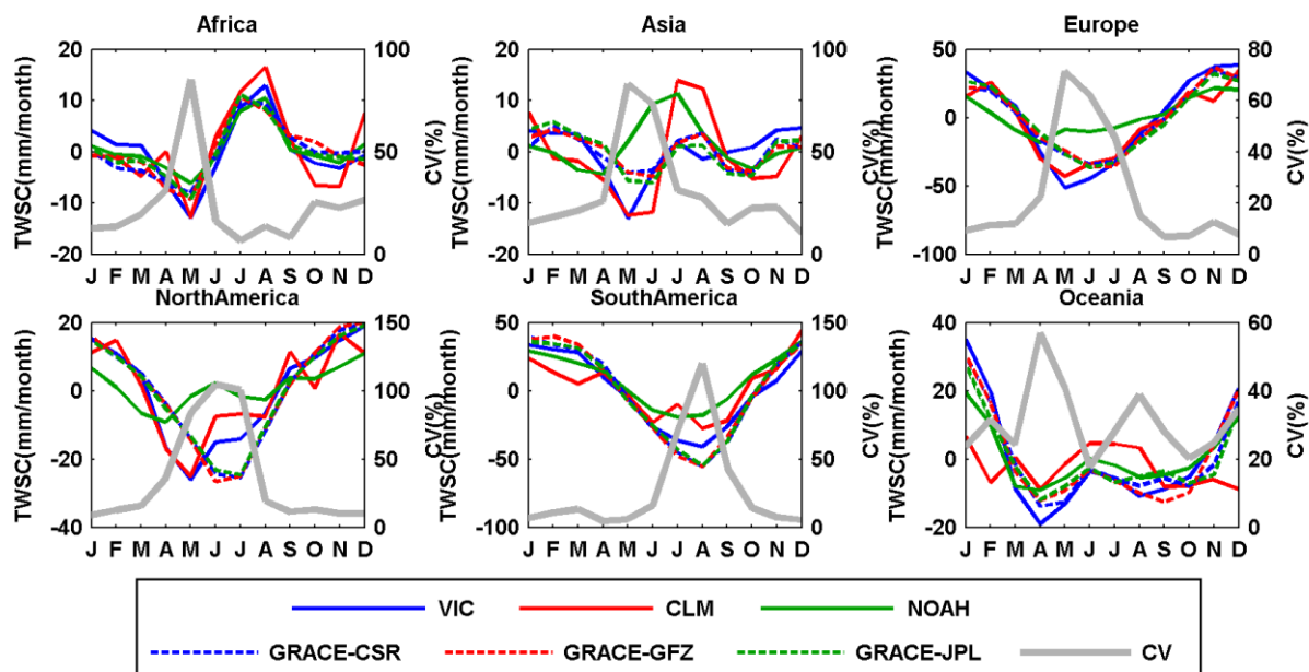
Figure 8. Seasonal cycles of total water storage change (TWSC) from different products over the six continents for 2003-2010
