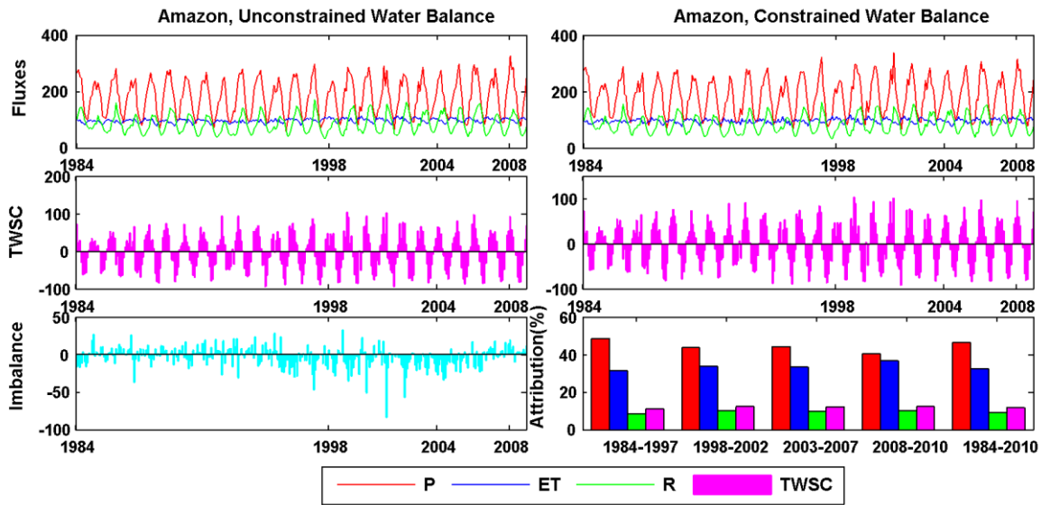
Figure 13. Unconstrained (left column) and constrained (right column) water budget estimates (mm/month) over Amazon River basin. The top, middle and bottom rows show the time series of water budget in terms of fluxes (precipitation, evapotranspiration and runoff), TWSC (Total Water Storage Change) and Imbalance. The imbalance/non-closure error after water budget constraint equals to zero and the imbalance/non-closure attributions to each water budget variables throughout different sub-periods are shown at the right bottom.
