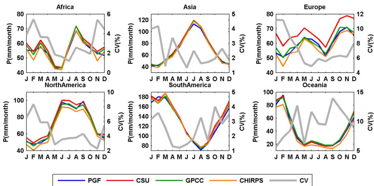
Figure 2. Seasonal cycles of precipitation from different products over the six continents for 1998-2010 (CHIRPS and CSU only cover the region between 50°N-50°S; therefore, only the grids between 50°N-50°S are counted into the calculation of the seasonal cycle; the Coefficient of Variance (CV, %) is calculated as the standard deviation divided by the ensemble mean of all the products (The same for Figures 3-9))
