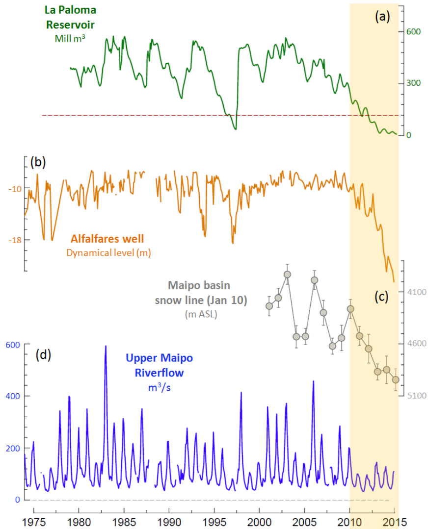
5 Figure 9. Selected hydrological impacts of the MD (highlighted by the yellow area). (a) Green curve: Monthly mean water volume in the La Paloma reservoir (32°S). (b) Orange curve: Monthly mean water depth in the Alfalfares observation well (32.5°S). (c) Grey curve: January 10th (early summer) height of the snowline between 33-34°S (note that the scale has been reversed). (d) Blue curve: Monthly mean Maipo river flow as measures in station El Manzano (850 m ASL, 33.5°S).
