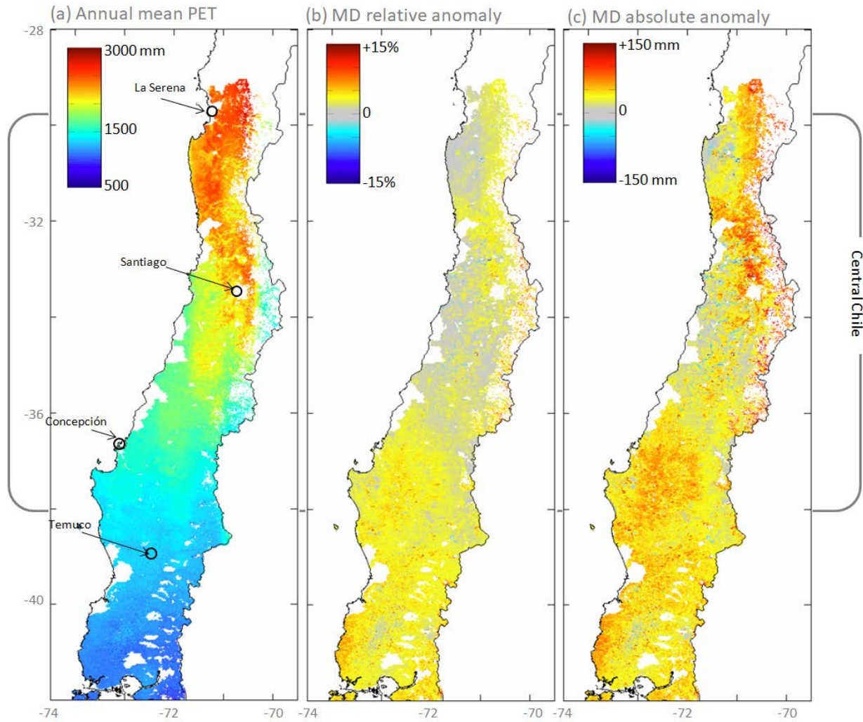
Figure 11. (a) Annual mean MODIS-derived potential evapotranspiration (PET) over Central Chile (2001-2015). (b) MD-averaged PET anomalies relative to the long-term mean. (c) MD-averaged PET absolute anomalies.
