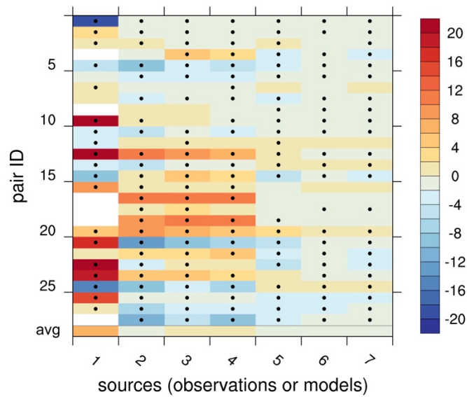
Figure S2. Same as Figure 13, but for the change in observed and simulated daytime surface soil moisture (%) during local summer.
