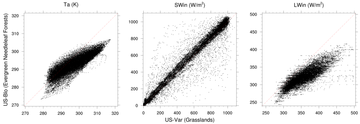
Figure S1. Comparison of air temperature (K, left), downwelling shortwave (middle) and longwave (right) radiations ( W/m^2 ) between the paired sites No. 15. The horizontal axis shows the observations from the grassland site US-Var, and the vertical axis shows the observations from the evergreen needleleaf forest site US-Blo.
