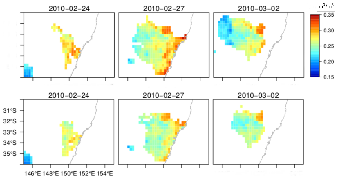
Figure 13. Sample drought event for February 2010, showing only the root zone soil moisture below the 10 % quantile level for the open-loop (above) and experiment DA 2 (below). The different spatial extent and differences in soil moisture itself, depending on the dataset used, at three different days are clearly visible. The figure is centred around the Central coast of New South Wales.
