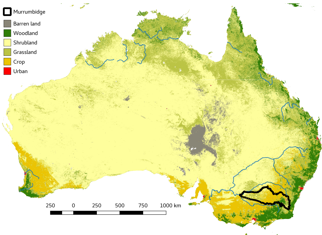
Figure 1. CLM plant functional types based on MODIS MCDQ12 land cover classification and ECOCLIMAP climate zones at 500 m resolution prior to the aggregation to 0.25 degrees. Some classes are here aggregated for visualisation purpose, e.g. evergreen temperate and evergreen tropical forests are both shown as Woodland. The boundary of the Murrumbidgee catchment, which is the site of the OzNet in-situ measurements, is shown.
