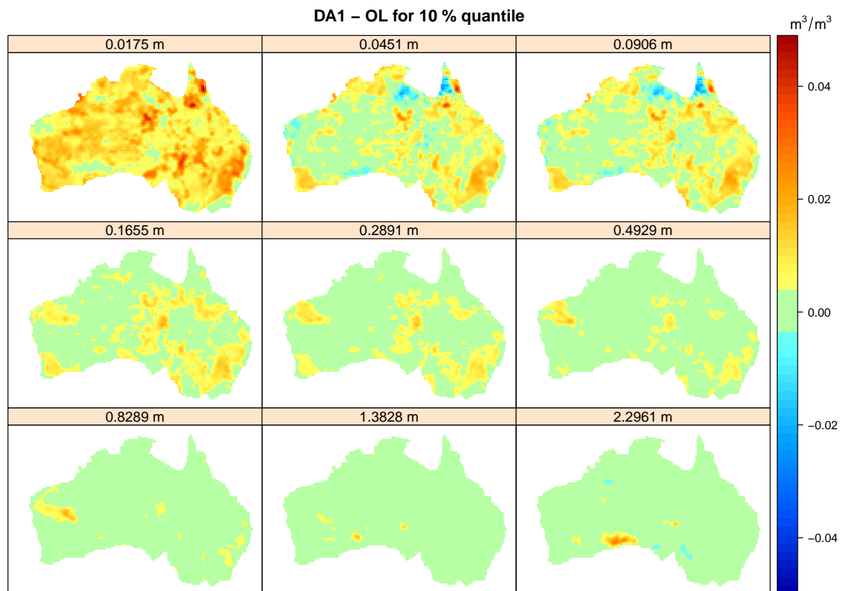
Figure 10. Differences in relative soil moisture between open-loop and DA 1 experiment (DA 1 - OL) for 10 % quantile. The individual panels correspond to the top 9 CLM soil layers titled with their depth.
