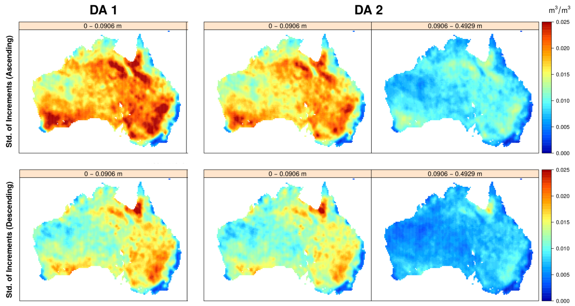
Figure 7. Standard deviation of increments for experiment DA 1 / DA 2 for top-layer soil moisture and root zone soil moisture for ascending (above) and descending orbits (below). Increments are strongest for the ascending orbit and for top-layer soil moisture and even stronger when restricting assimilation to these layers, as in DA 1. Increments are very low or zero for the forested areas along the coastline, either due to the absence of observations or the high LAI values masking any soil moisture signal within the forward operator.
