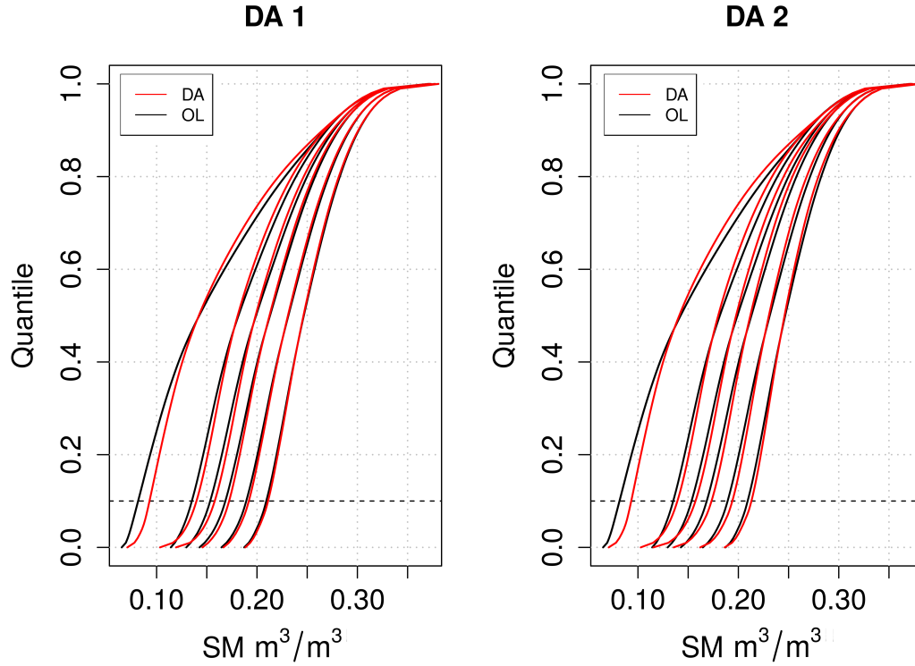
Figure 12. Cumulative distribution functions (CDFs) for the upper 6 CLM soil layers for experiments DA 1 and DA 2, based on quantiles computed for all data across the model domain. CDFs for open-loop simulations are shown in black and assimilation results in red. Both panels show changes in CDF behaviour for the layers being updated in the respective experiments, i.e. layers 1-3 for DA 1 and layers 1-6 for DA 2. Soil moisture increases systematically with soil depth allowing for the easy identification of the layers within the plot. The dashed vertical line marks the 10 % quantile, corresponding to figures 10 and 11.
