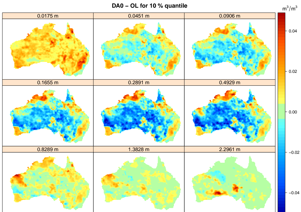
Figure 9. Differences in relative soil moisture between open-loop and DA 0 experiment (DA 0 - OL) for the 10 % quantile. The individual panels correspond to the top 9 CLM soil layers.
