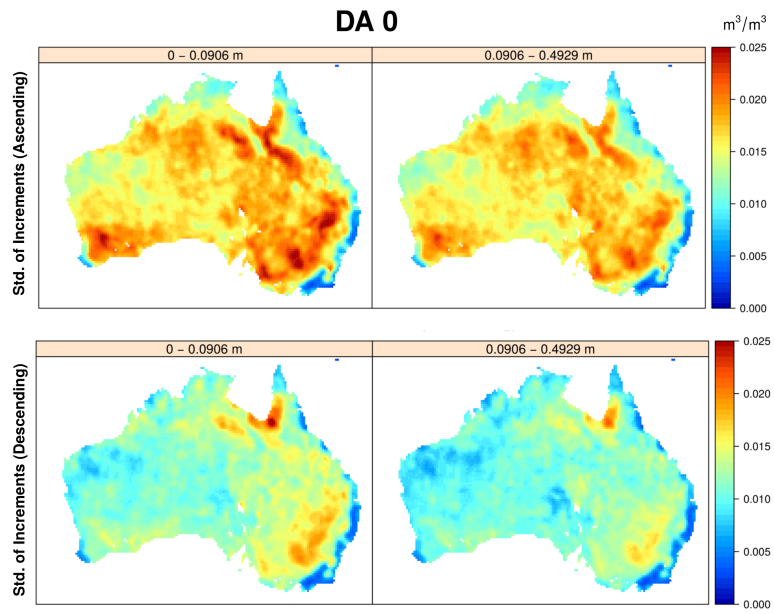
Figure 5. Increments standard deviation of all increments for experiment DA 0 for top-layer soil moisture (left) and root-zone soil moisture (right) for ascending (above) and descending orbits (below). Increments for the root-zone soil moisture are fairly similar to the top soil layers, due to the homogeneous texture perturbations applied across all layers.
