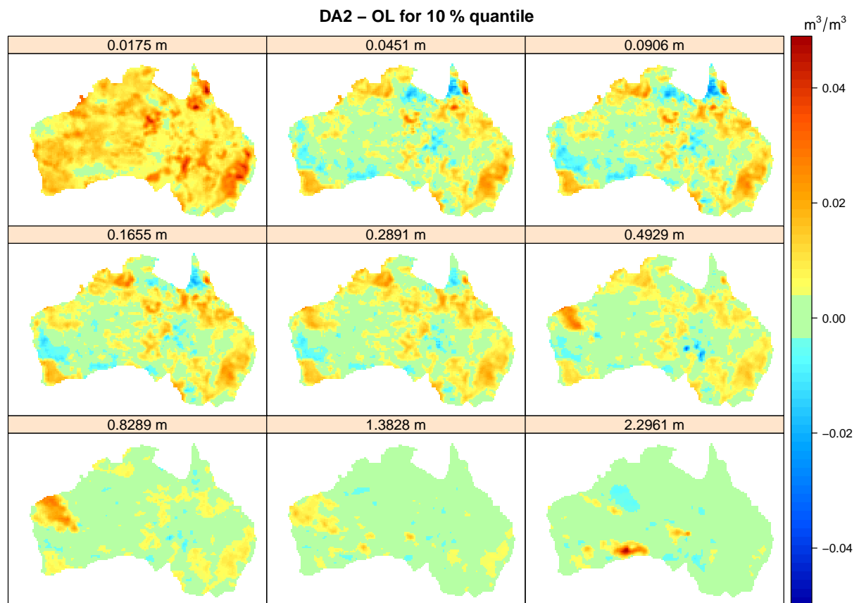
Figure 11. Differences in relative soil moisture between open-loop and DA 2 experiment (DA 2 - OL) for the 10 % quantile. The individual panels correspond to the top 9 CLM soil layers.
