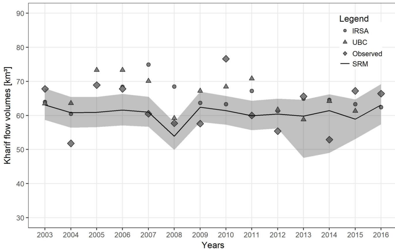
Figure 12: Comparison of Kharif flow forecasts with 20% and 80% quantiles of SRM+G scenario ensembles years 2003 - 2016
