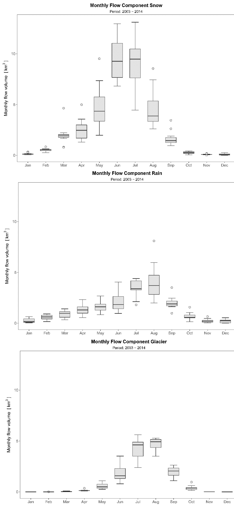
Figure 7: Monthly distribution of flow components in UIB
